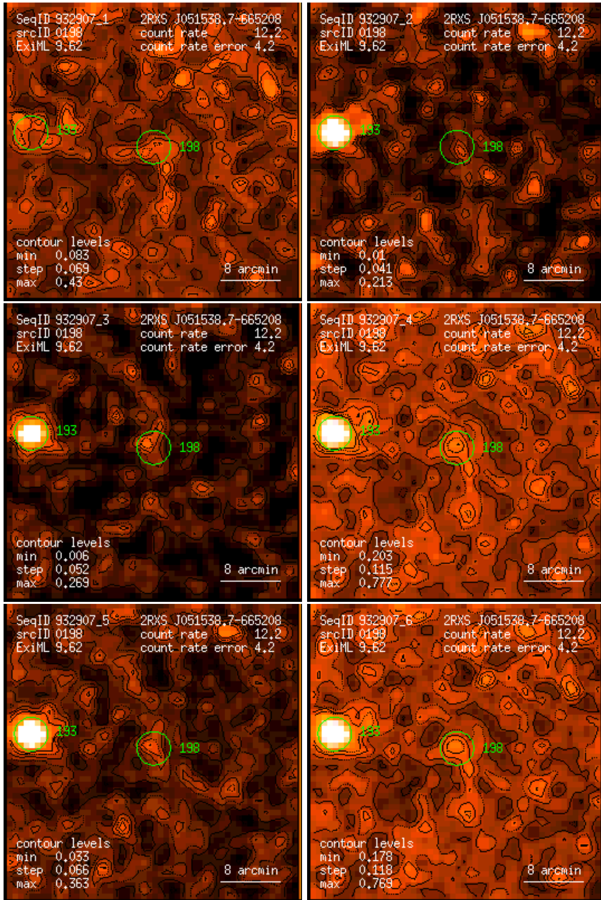
Figure 198: RASS 932907: detection 0198: band rate images, Gaussian filter: (1) PSPC channels 11 – 41, (2) 52 – 90, (3) 91 – 201, (4) 11 – 235, (5) 52 – 201, (6) 11 – 201. Broad band rates in counts/ks. Band rate contour levels in counts/ks/arcmin 2 .
