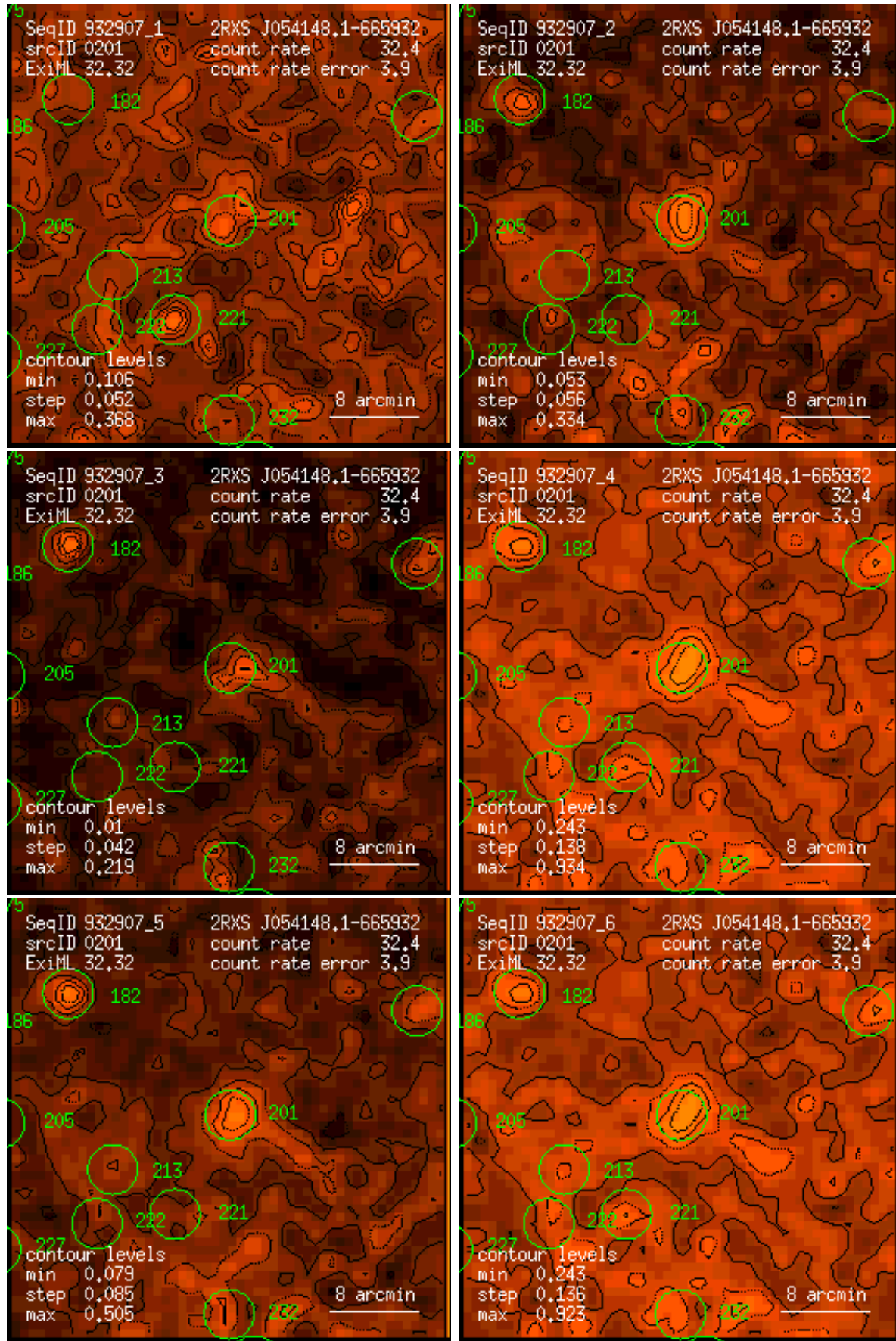
Figure 201: RASS 932907: detection 0201: band rate images, Gaussian filter: (1) PSPC channels 11 – 41, (2) 52 – 90, (3) 91 – 201, (4) 11 – 235, (5) 52 – 201, (6) 11 – 201. Broad band rates in counts/ks. Band rate contour levels in counts/ks/arcmin 2 .
