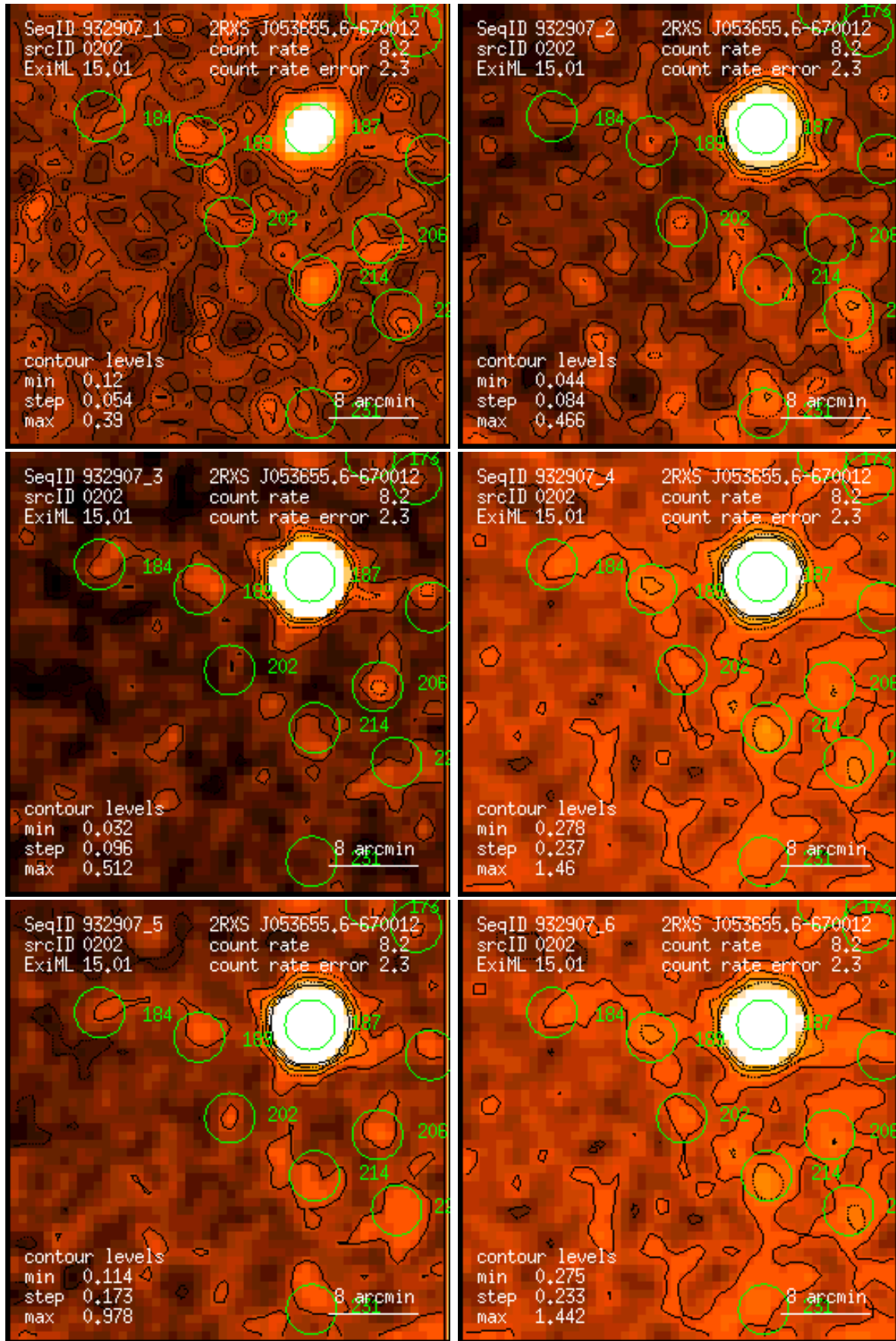
Figure 202: RASS 932907: detection 0202: band rate images, Gaussian filter: (1) PSPC channels 11 – 41, (2) 52 – 90, (3) 91 – 201, (4) 11 – 235, (5) 52 – 201, (6) 11 – 201. Broad band rates in counts/ks. Band rate contour levels in counts/ks/arcmin 2 .
