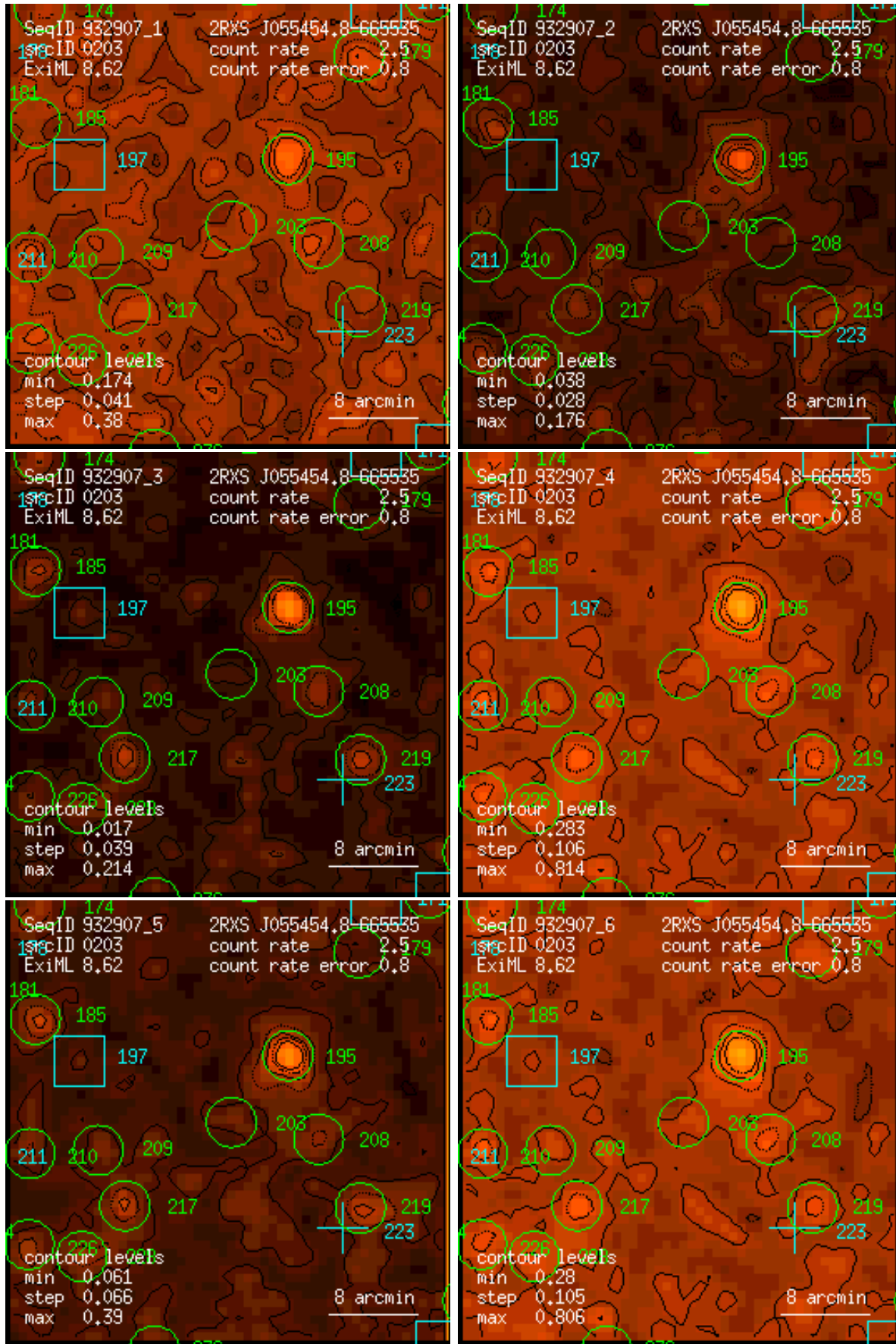
Figure 203: RASS 932907: detection 0203: band rate images, Gaussian filter: (1) PSPC channels 11 – 41, (2) 52 – 90, (3) 91 – 201, (4) 11 – 235, (5) 52 – 201, (6) 11 – 201. Broad band rates in counts/ks. Band rate contour levels in counts/ks/arcmin 2 .
