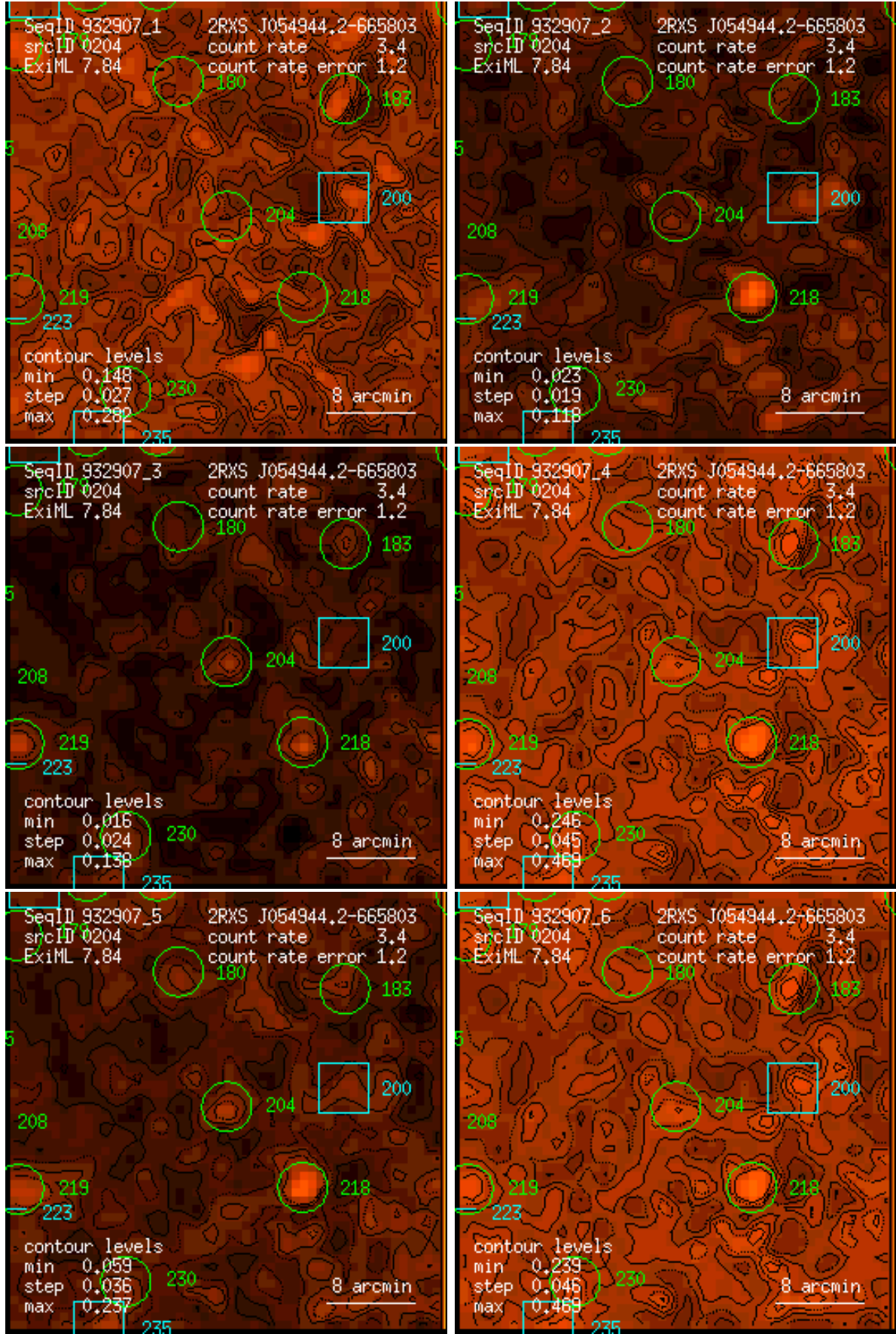
Figure 204: RASS 932907: detection 0204: band rate images, Gaussian filter: (1) PSPC channels 11 – 41, (2) 52 – 90, (3) 91 – 201, (4) 11 – 235, (5) 52 – 201, (6) 11 – 201. Broad band rates in counts/ks. Band rate contour levels in counts/ks/arcmin 2 .
