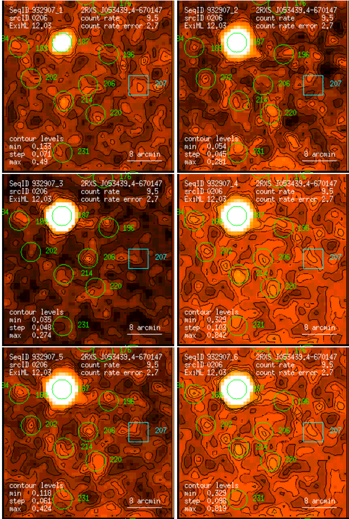
Figure 206: RASS 932907: detection 0206: band rate images, Gaussian filter: (1) PSPC channels 11 – 41, (2) 52 – 90, (3) 91 – 201, (4) 11 – 235, (5) 52 – 201, (6) 11 – 201. Broad band rates in counts/ks. Band rate contour levels in counts/ks/arcmin 2 .
