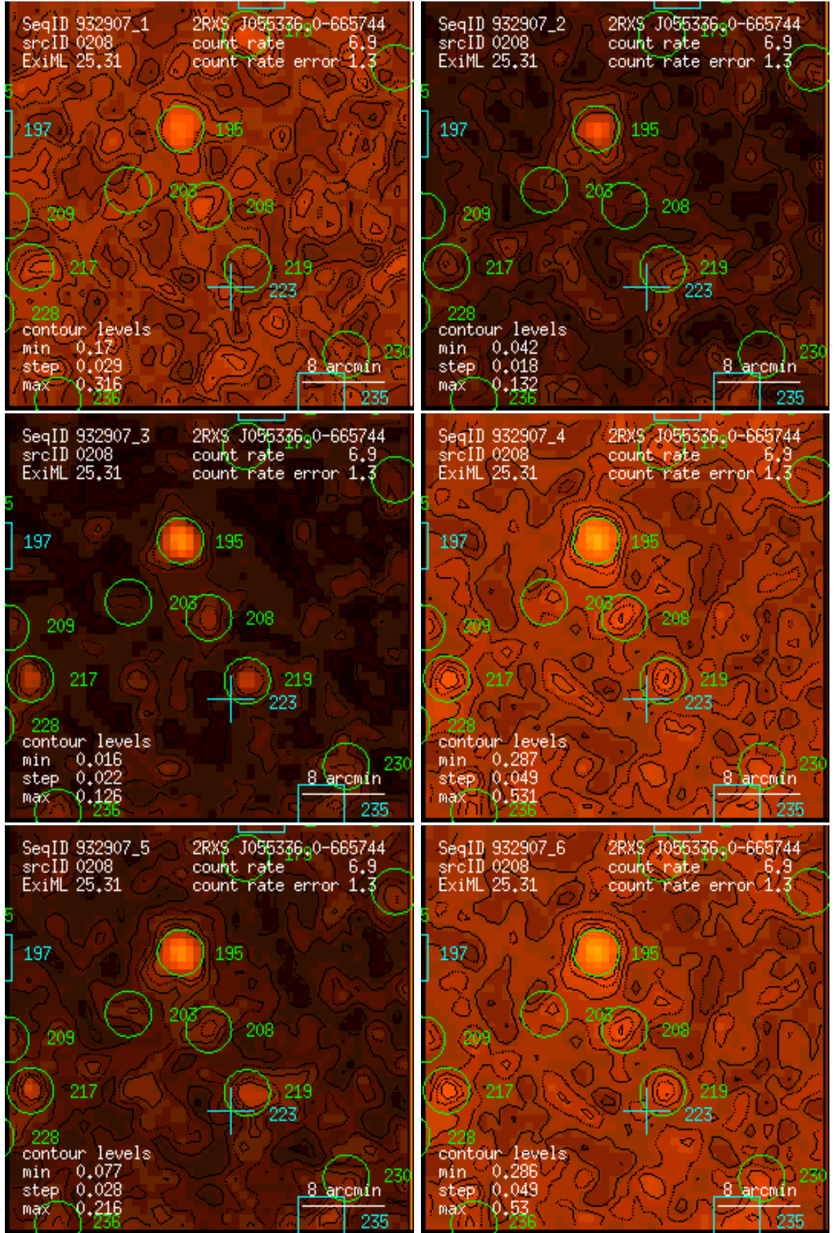
Figure 208: RASS 932907: detection 0208: band rate images, Gaussian filter: (1) PSPC channels 11 – 41, (2) 52 – 90, (3) 91 – 201, (4) 11 – 235, (5) 52 – 201, (6) 11 – 201. Broad band rates in counts/ks. Band rate contour levels in counts/ks/arcmin 2 .
