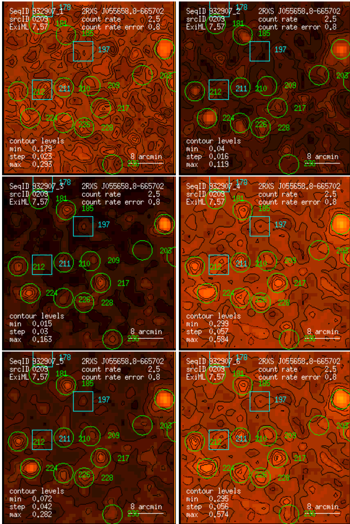
Figure 209: RASS 932907: detection 0209: band rate images, Gaussian filter: (1) PSPC channels 11 – 41, (2) 52 – 90, (3) 91 – 201, (4) 11 – 235, (5) 52 – 201, (6) 11 – 201. Broad band rates in counts/ks. Band rate contour levels in counts/ks/arcmin 2 .
