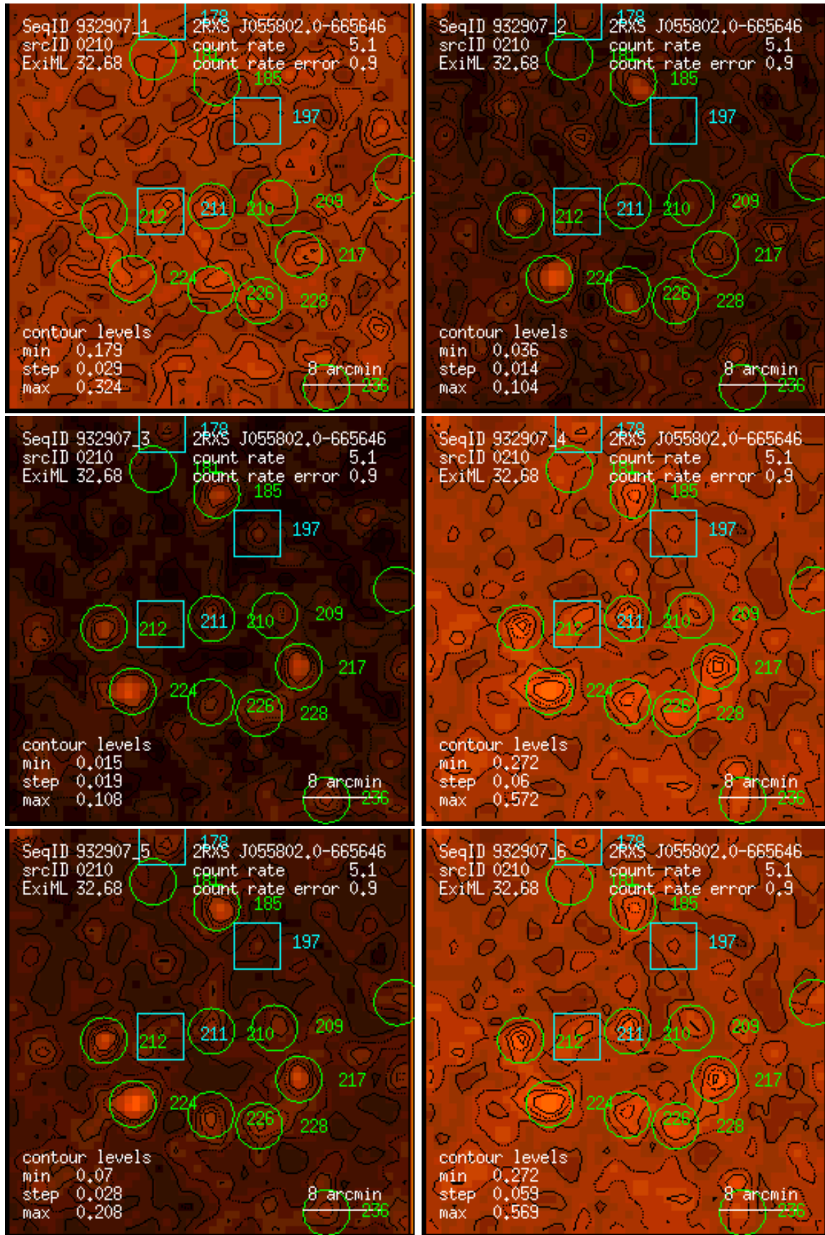
Figure 210: RASS 932907: detection 0210: band rate images, Gaussian filter: (1) PSPC channels 11 – 41, (2) 52 – 90, (3) 91 – 201, (4) 11 – 235, (5) 52 – 201, (6) 11 – 201. Broad band rates in counts/ks. Band rate contour levels in counts/ks/arcmin 2 .
