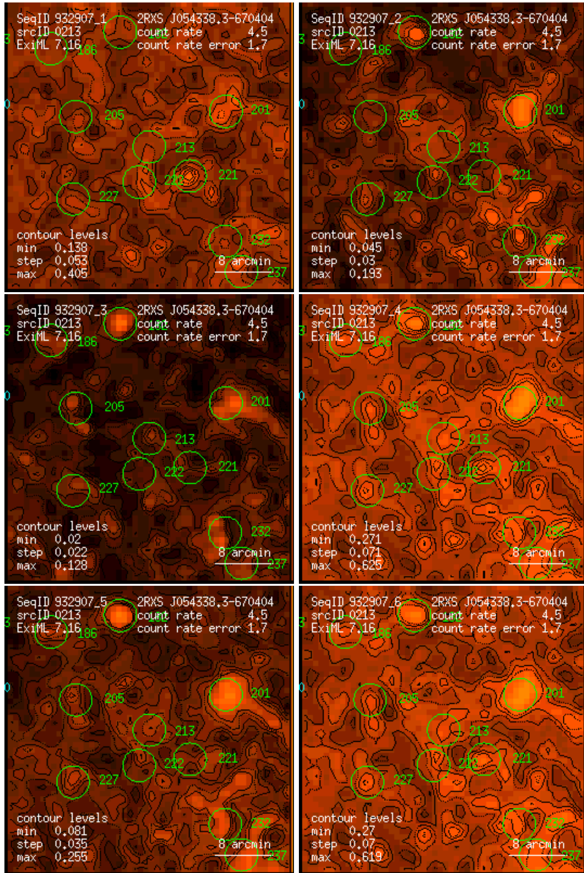
Figure 213: RASS 932907: detection 0213: band rate images, Gaussian filter: (1) PSPC channels 11 – 41, (2) 52 – 90, (3) 91 – 201, (4) 11 – 235, (5) 52 – 201, (6) 11 – 201. Broad band rates in counts/ks. Band rate contour levels in counts/ks/arcmin 2 .
