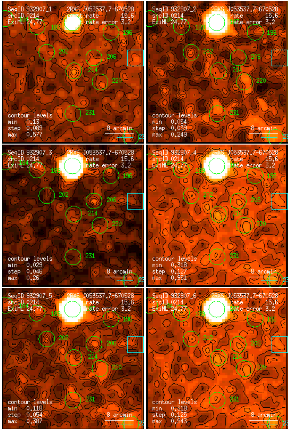
Figure 214: RASS 932907: detection 0214: band rate images, Gaussian filter: (1) PSPC channels 11 – 41, (2) 52 – 90, (3) 91 – 201, (4) 11 – 235, (5) 52 – 201, (6) 11 – 201. Broad band rates in counts/ks. Band rate contour levels in counts/ks/arcmin 2 .
