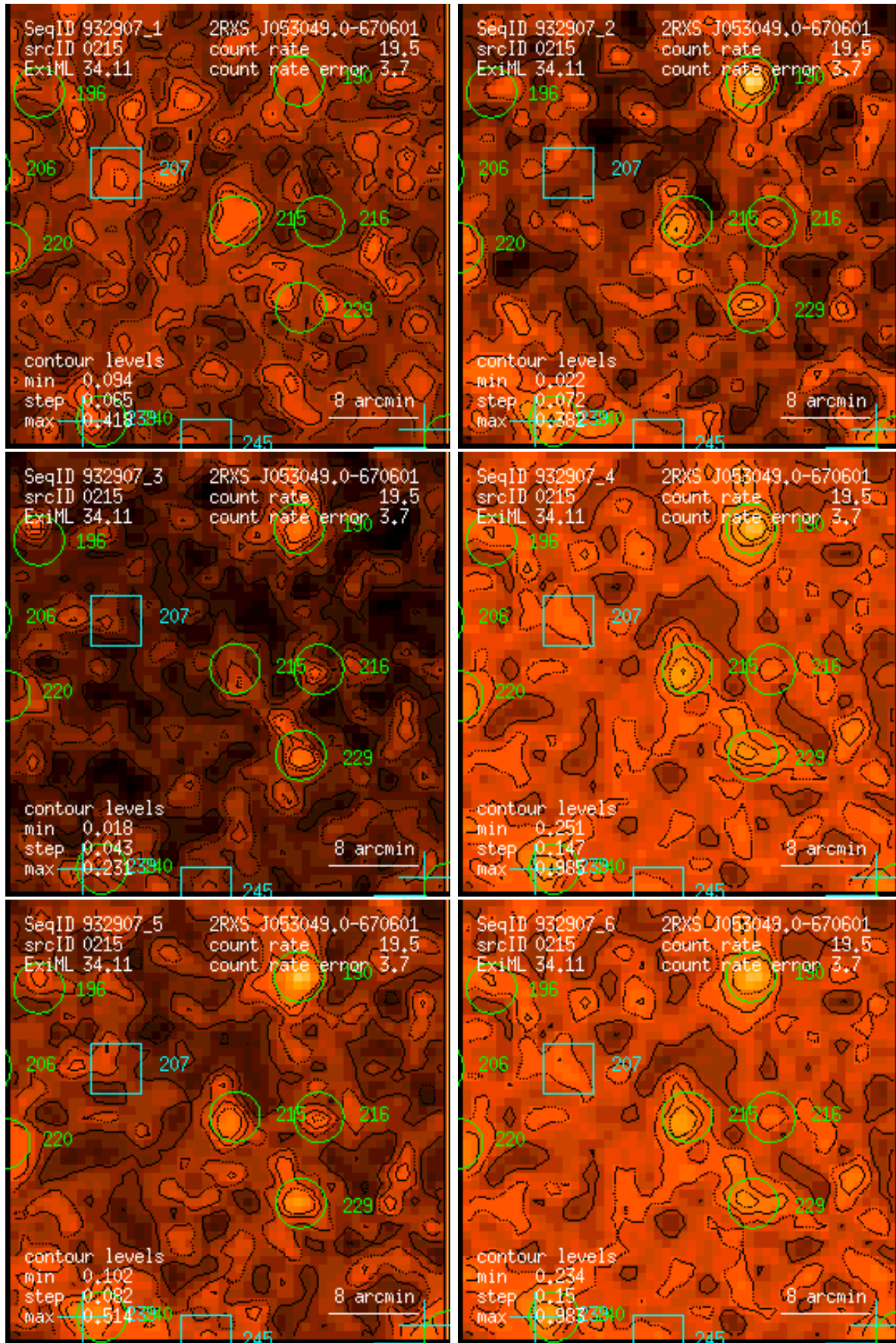
Figure 215: RASS 932907: detection 0215: band rate images, Gaussian filter: (1) PSPC channels 11 – 41, (2) 52 – 90, (3) 91 – 201, (4) 11 – 235, (5) 52 – 201, (6) 11 – 201. Broad band rates in counts/ks. Band rate contour levels in counts/ks/arcmin 2 .
