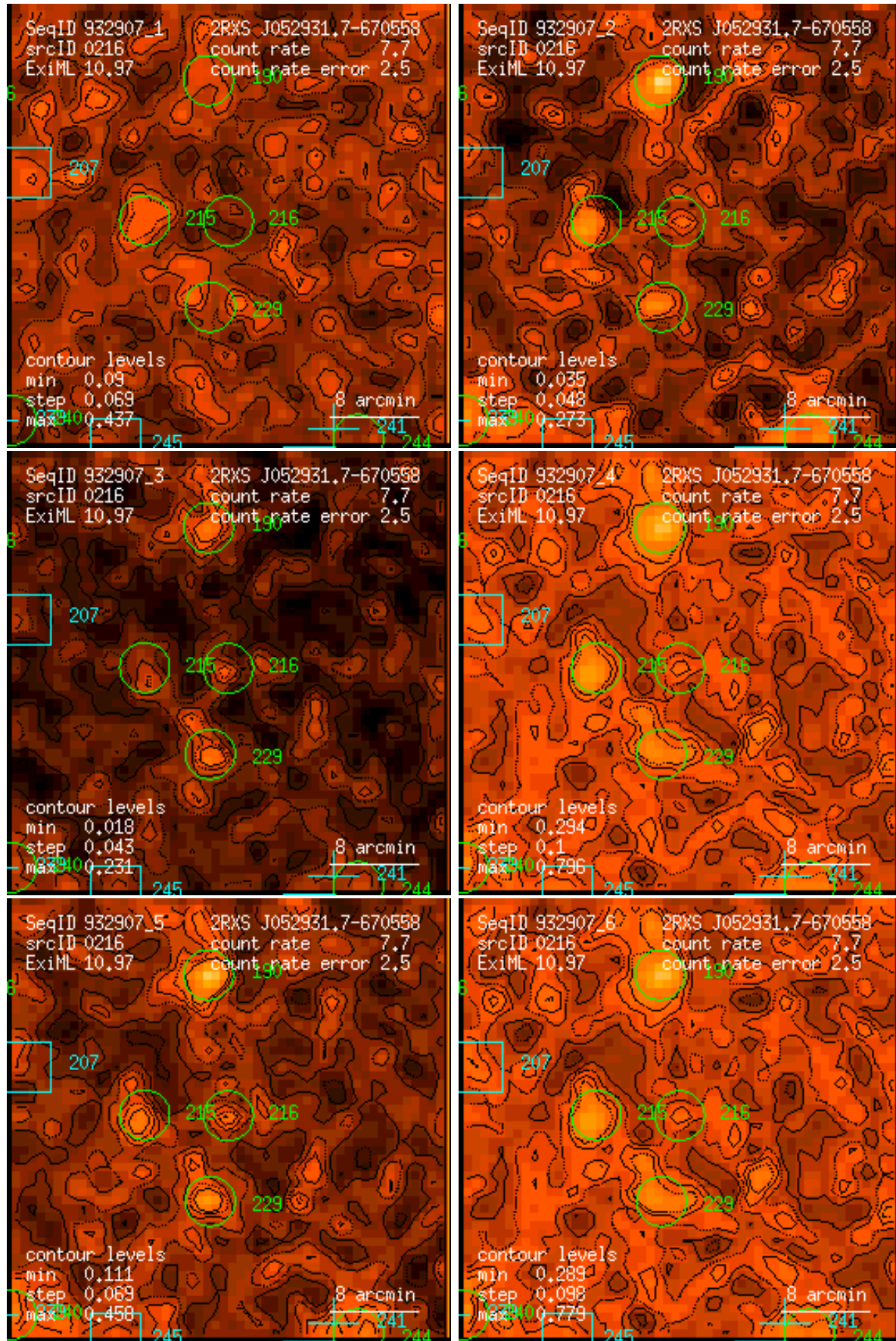
Figure 216: RASS 932907: detection 0216: band rate images, Gaussian filter: (1) PSPC channels 11 – 41, (2) 52 – 90, (3) 91 – 201, (4) 11 – 235, (5) 52 – 201, (6) 11 – 201. Broad band rates in counts/ks. Band rate contour levels in counts/ks/arcmin 2 .
