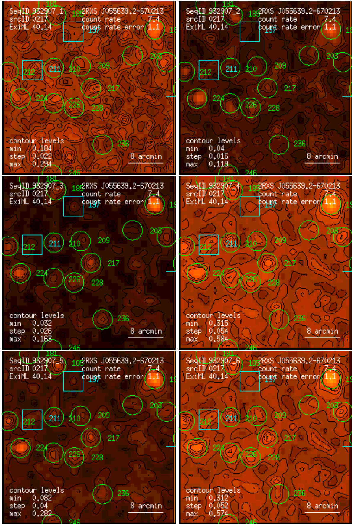
Figure 217: RASS 932907: detection 0217: band rate images, Gaussian filter: (1) PSPC channels 11 – 41, (2) 52 – 90, (3) 91 – 201, (4) 11 – 235, (5) 52 – 201, (6) 11 – 201. Broad band rates in counts/ks. Band rate contour levels in counts/ks/arcmin 2 .
