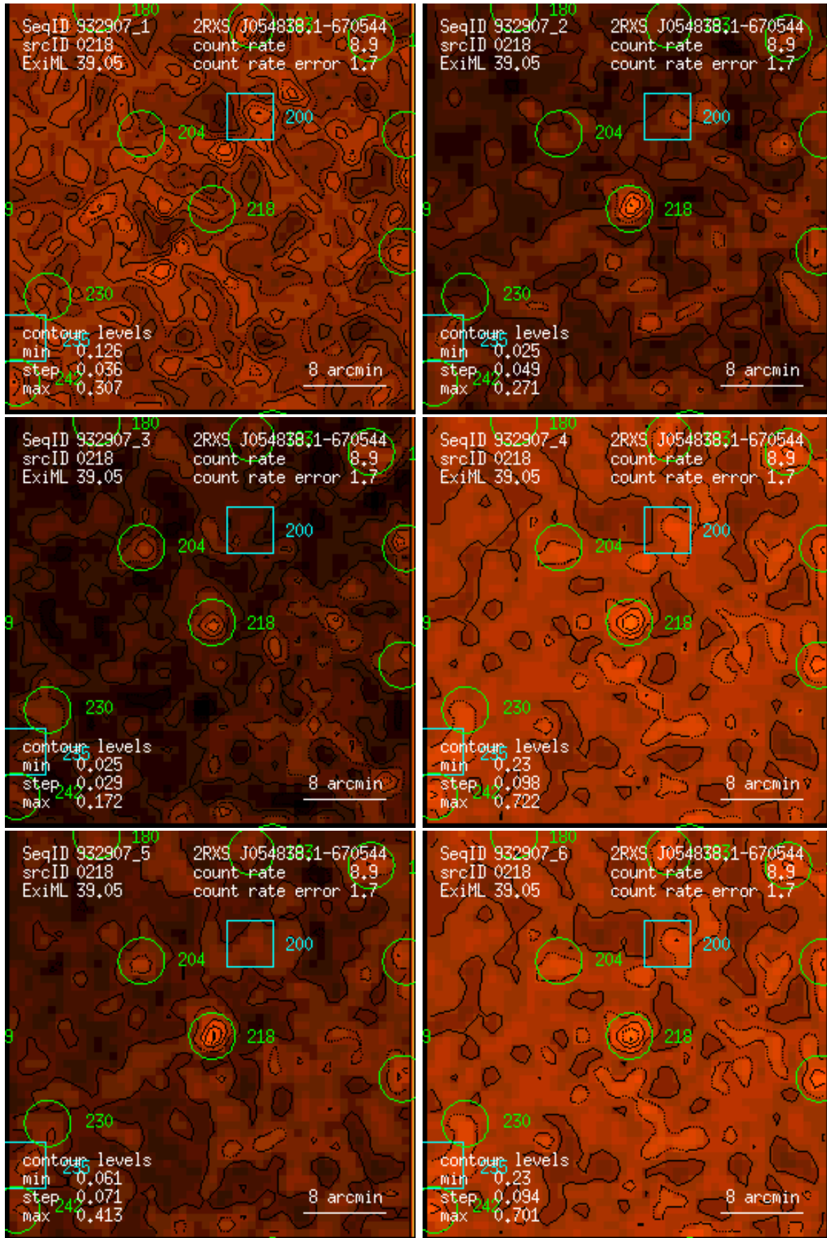
Figure 218: RASS 932907: detection 0218: band rate images, Gaussian filter: (1) PSPC channels 11 – 41, (2) 52 – 90, (3) 91 – 201, (4) 11 – 235, (5) 52 – 201, (6) 11 – 201. Broad band rates in counts/ks. Band rate contour levels in counts/ks/arcmin 2 .
