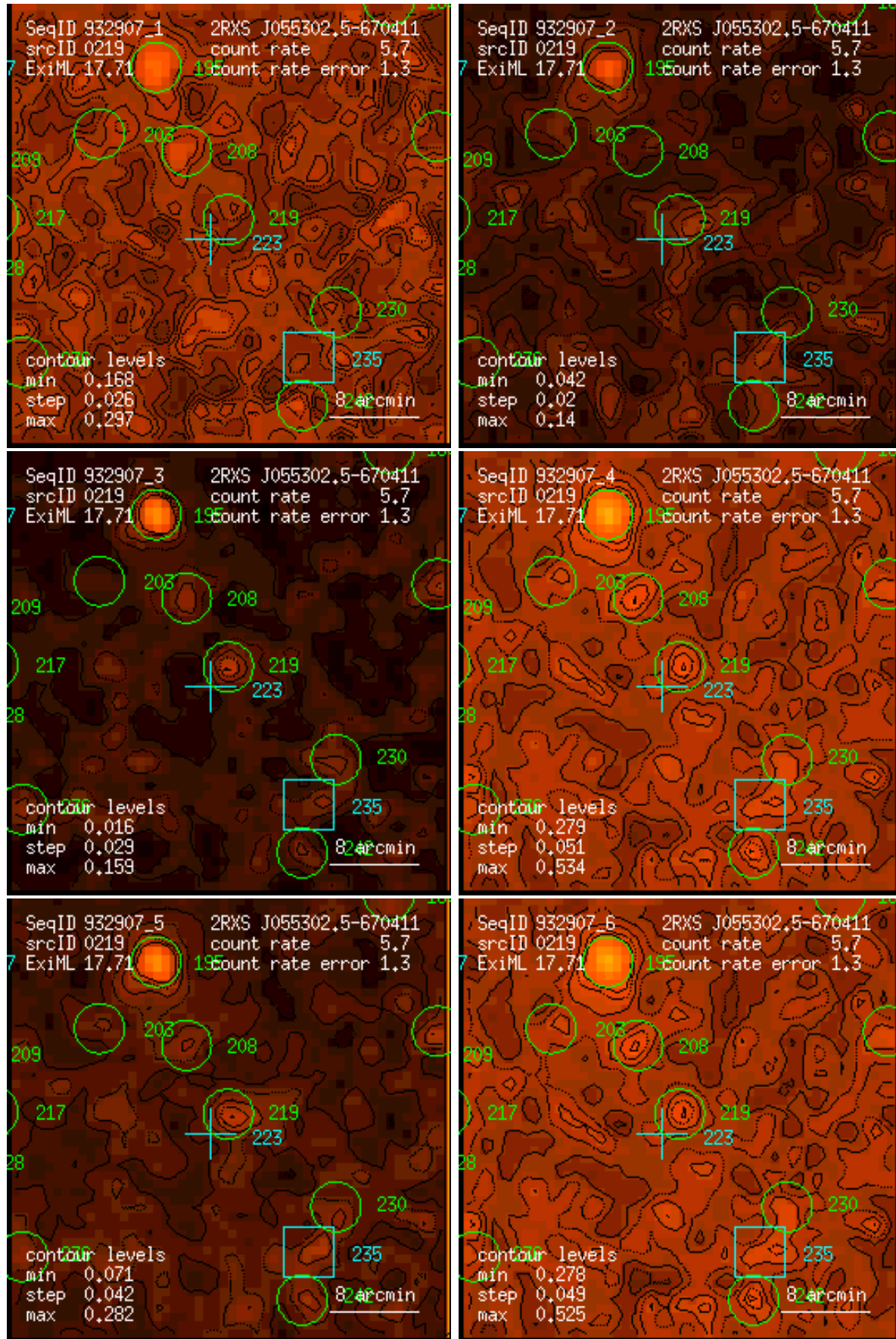
Figure 219: RASS 932907: detection 0219: band rate images, Gaussian filter: (1) PSPC channels 11 – 41, (2) 52 – 90, (3) 91 – 201, (4) 11 – 235, (5) 52 – 201, (6) 11 – 201. Broad band rates in counts/ks. Band rate contour levels in counts/ks/arcmin 2 .
