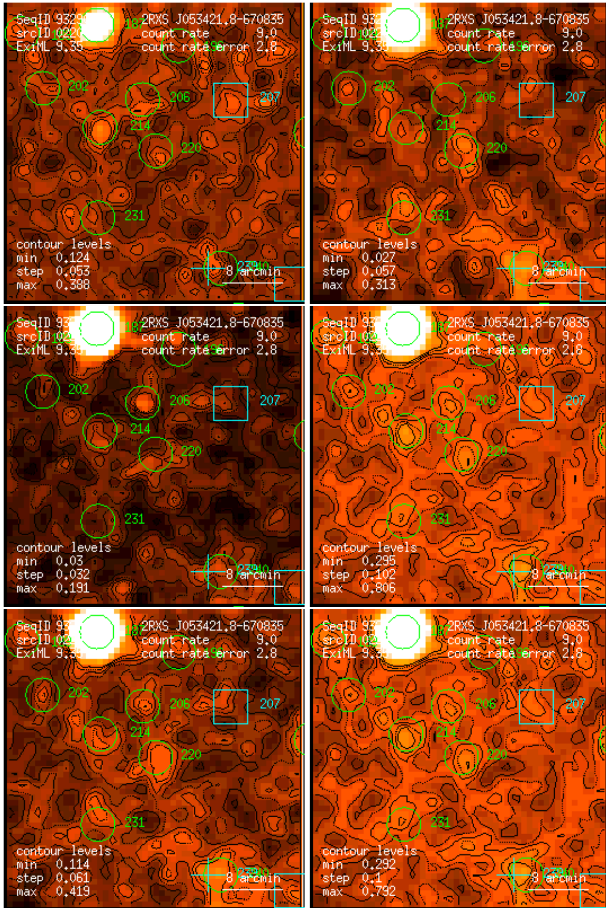
Figure 220: RASS 932907: detection 0220: band rate images, Gaussian filter: (1) PSPC channels 11 – 41, (2) 52 – 90, (3) 91 – 201, (4) 11 – 235, (5) 52 – 201, (6) 11 – 201. Broad band rates in counts/ks. Band rate contour levels in counts/ks/arcmin 2 .
