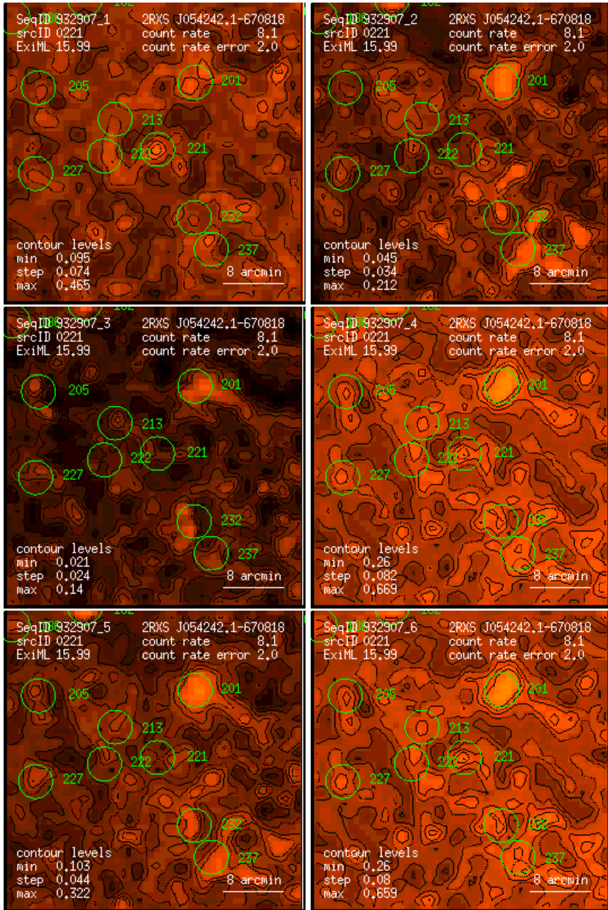
Figure 221: RASS 932907: detection 0221: band rate images, Gaussian filter: (1) PSPC channels 11 – 41, (2) 52 – 90, (3) 91 – 201, (4) 11 – 235, (5) 52 – 201, (6) 11 – 201. Broad band rates in counts/ks. Band rate contour levels in counts/ks/arcmin 2 .
