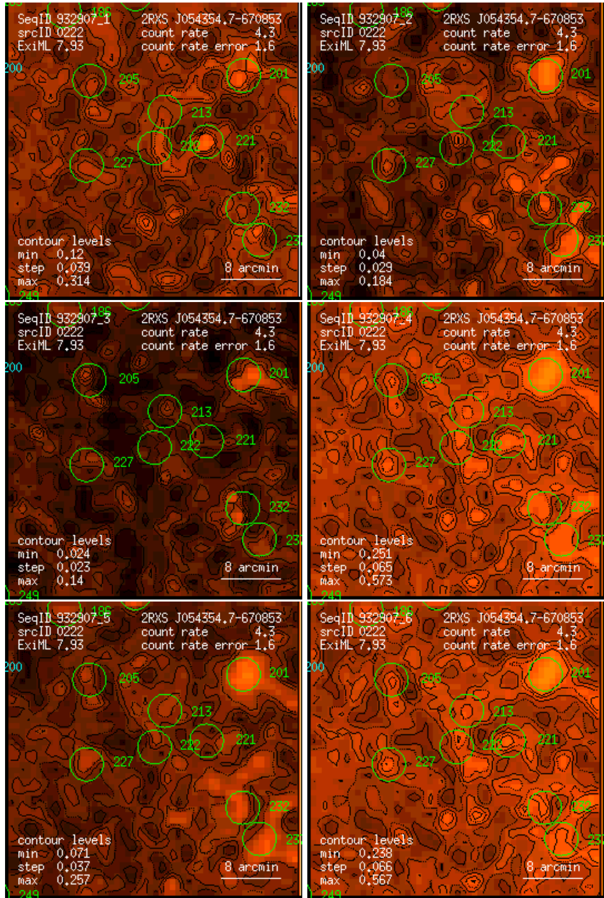
Figure 222: RASS 932907: detection 0222: band rate images, Gaussian filter: (1) PSPC channels 11 – 41, (2) 52 – 90, (3) 91 – 201, (4) 11 – 235, (5) 52 – 201, (6) 11 – 201. Broad band rates in counts/ks. Band rate contour levels in counts/ks/arcmin 2 .
