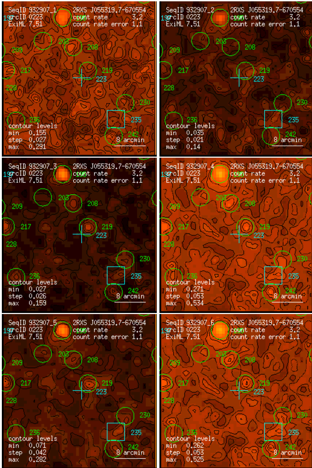
Figure 223: RASS 932907: detection 0223: band rate images, Gaussian filter: (1) PSPC channels 11 – 41, (2) 52 – 90, (3) 91 – 201, (4) 11 – 235, (5) 52 – 201, (6) 11 – 201. Broad band rates in counts/ks. Band rate contour levels in counts/ks/arcmin 2 .
