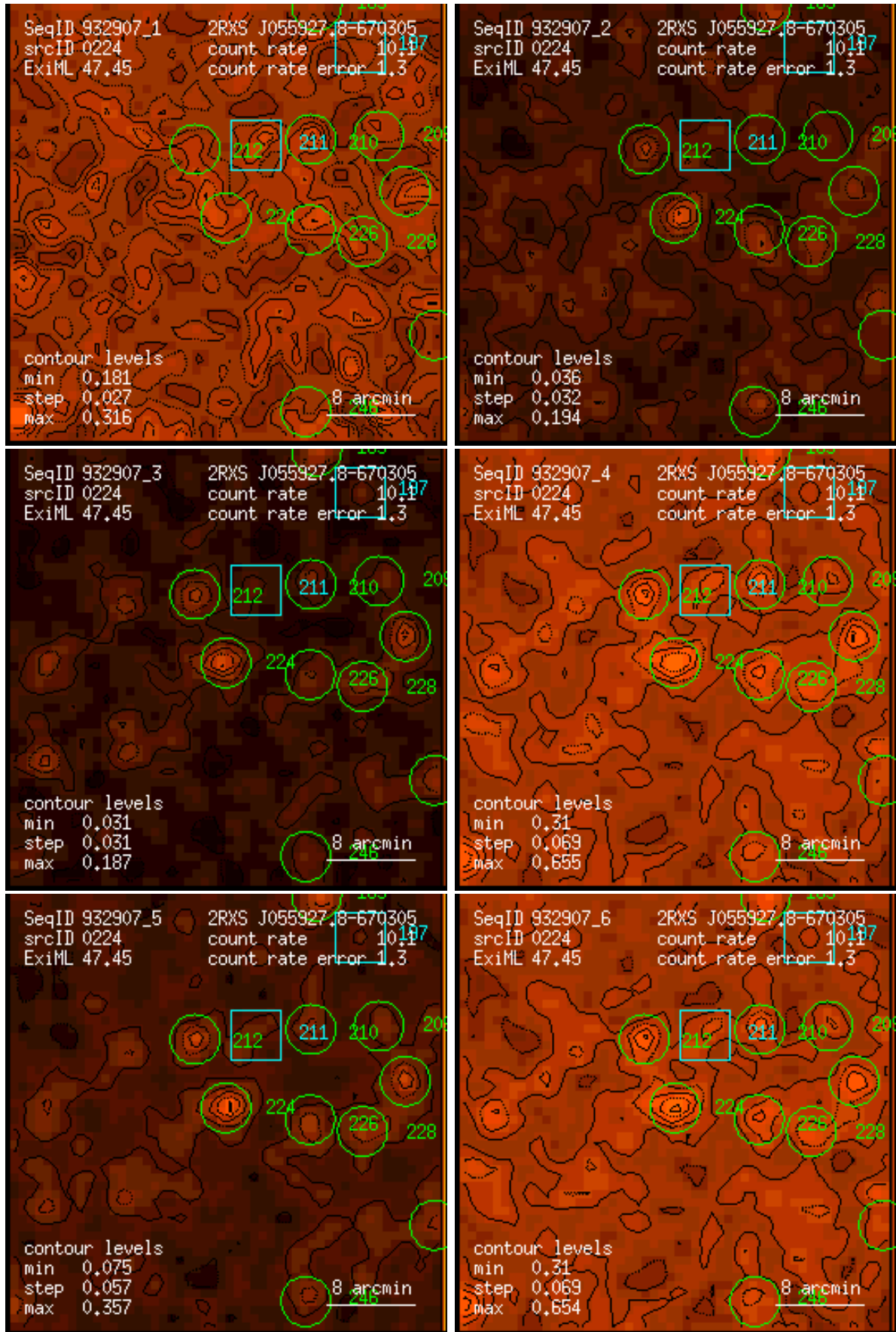
Figure 224: RASS 932907: detection 0224: band rate images, Gaussian filter: (1) PSPC channels 11 – 41, (2) 52 – 90, (3) 91 – 201, (4) 11 – 235, (5) 52 – 201, (6) 11 – 201. Broad band rates in counts/ks. Band rate contour levels in counts/ks/arcmin 2 .
