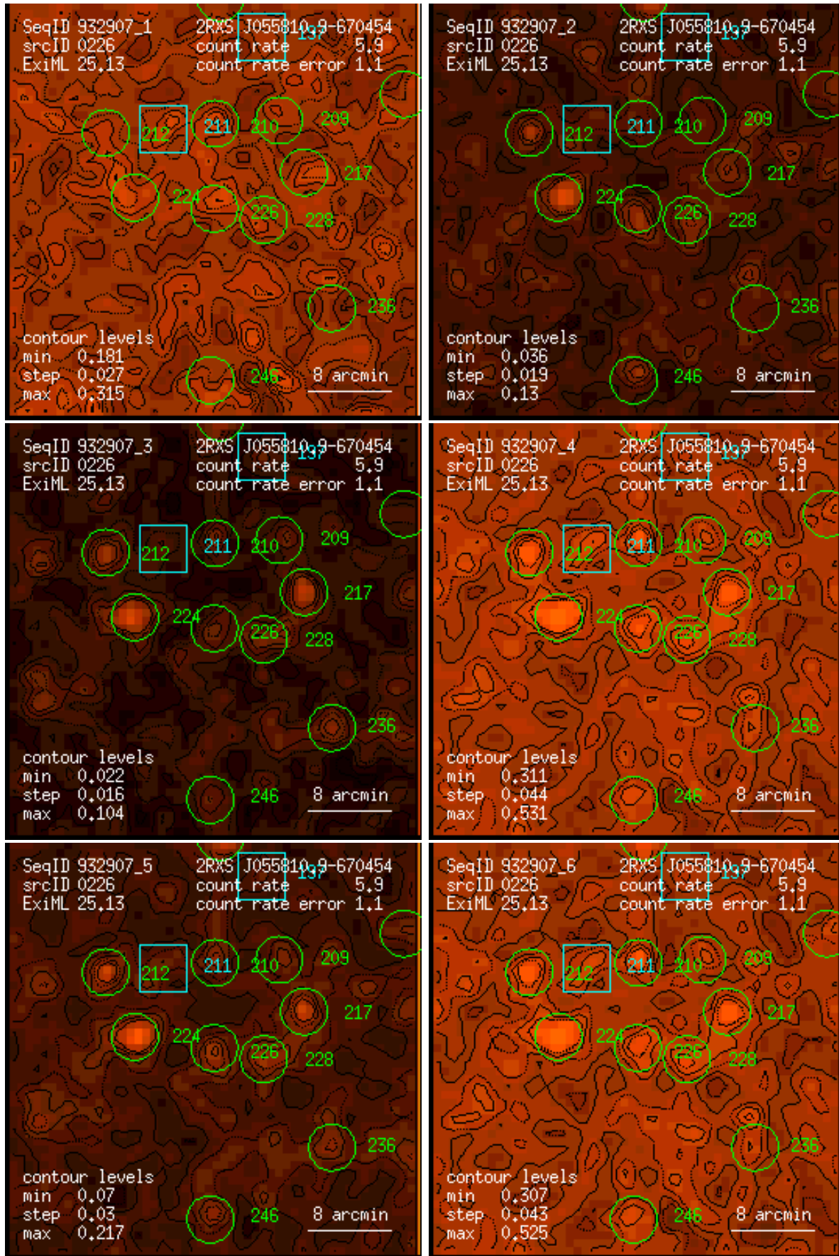
Figure 226: RASS 932907: detection 0226: band rate images, Gaussian filter: (1) PSPC channels 11 – 41, (2) 52 – 90, (3) 91 – 201, (4) 11 – 235, (5) 52 – 201, (6) 11 – 201. Broad band rates in counts/ks. Band rate contour levels in counts/ks/arcmin 2 .
