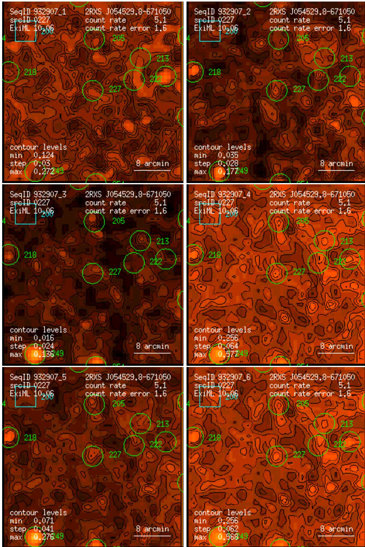
Figure 227: RASS 932907: detection 0227: band rate images, Gaussian filter: (1) PSPC channels 11 – 41, (2) 52 – 90, (3) 91 – 201, (4) 11 – 235, (5) 52 – 201, (6) 11 – 201. Broad band rates in counts/ks. Band rate contour levels in counts/ks/arcmin 2 .
