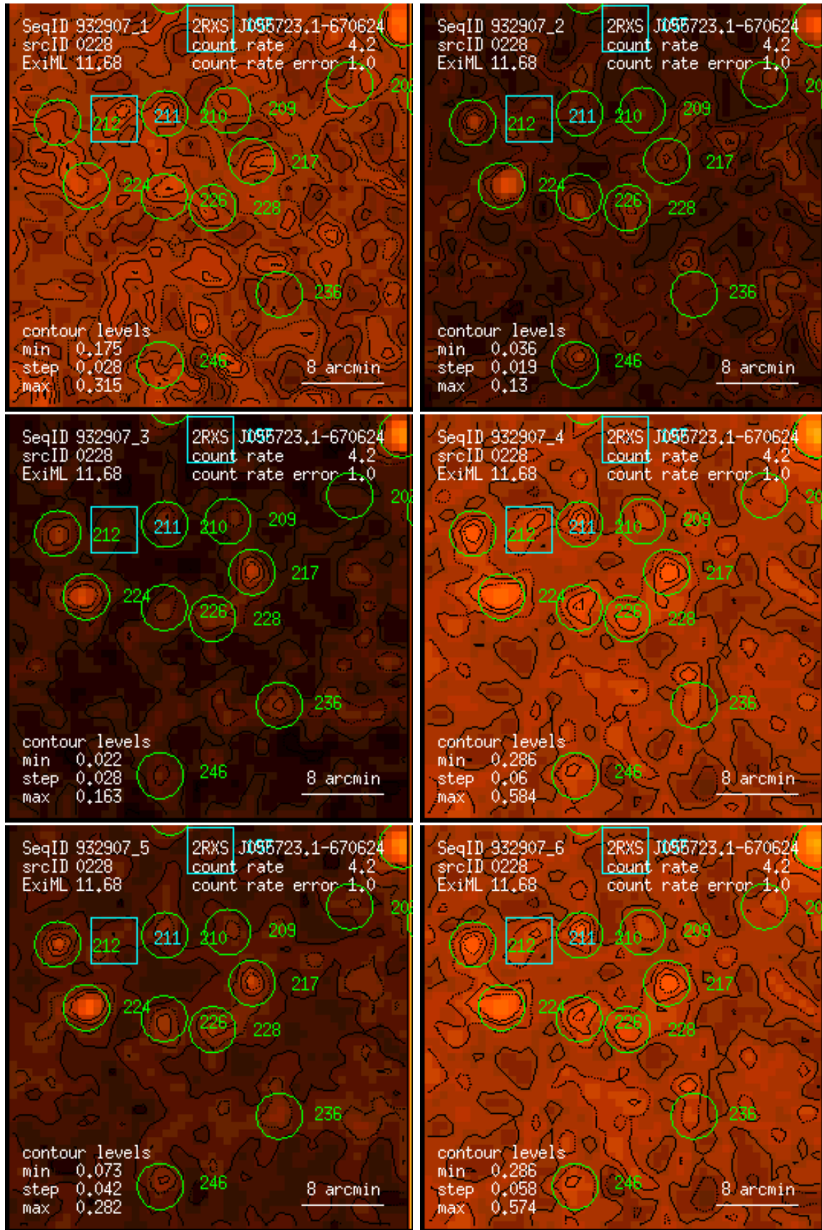
Figure 228: RASS 932907: detection 0228: band rate images, Gaussian filter: (1) PSPC channels 11 – 41, (2) 52 – 90, (3) 91 – 201, (4) 11 – 235, (5) 52 – 201, (6) 11 – 201. Broad band rates in counts/ks. Band rate contour levels in counts/ks/arcmin 2 .
