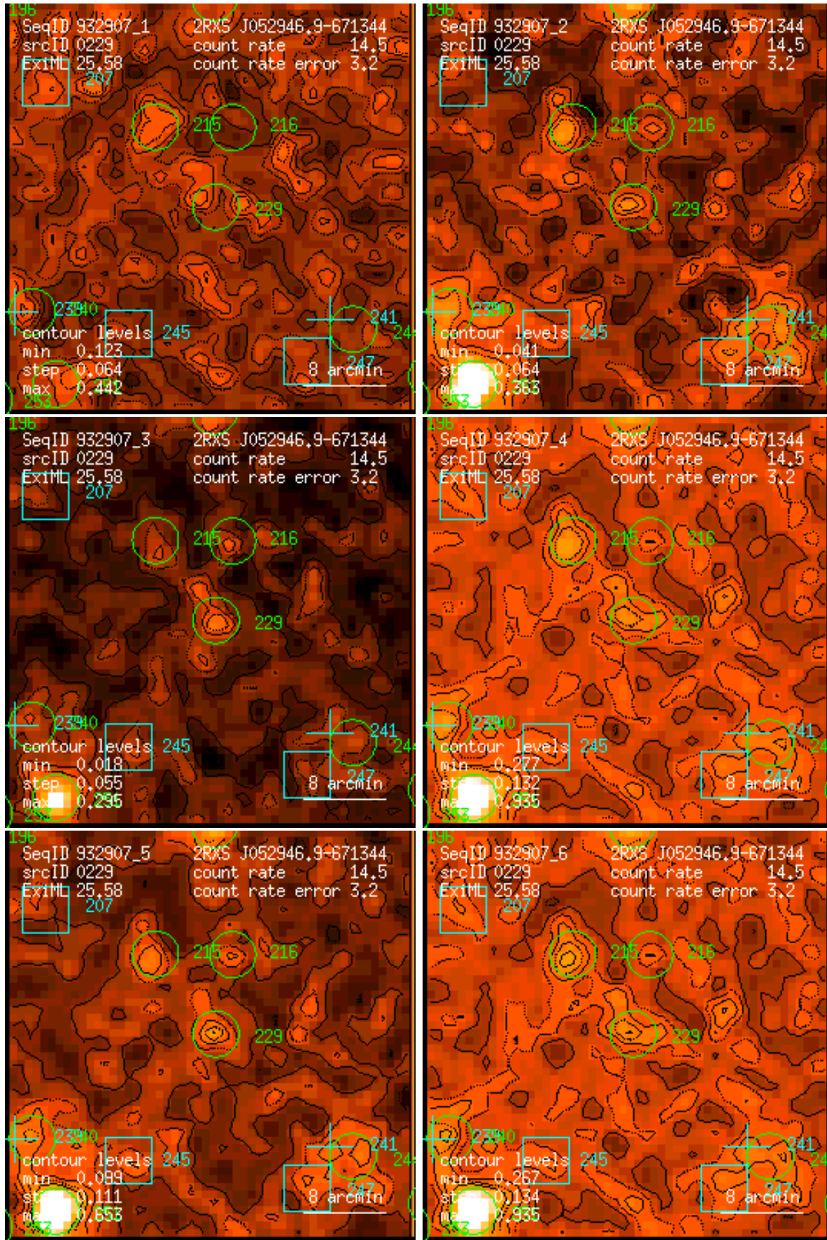
Figure 229: RASS 932907: detection 0229: band rate images, Gaussian filter: (1) PSPC channels 11 – 41, (2) 52 – 90, (3) 91 – 201, (4) 11 – 235, (5) 52 – 201, (6) 11 – 201. Broad band rates in counts/ks. Band rate contour levels in counts/ks/arcmin 2 .
