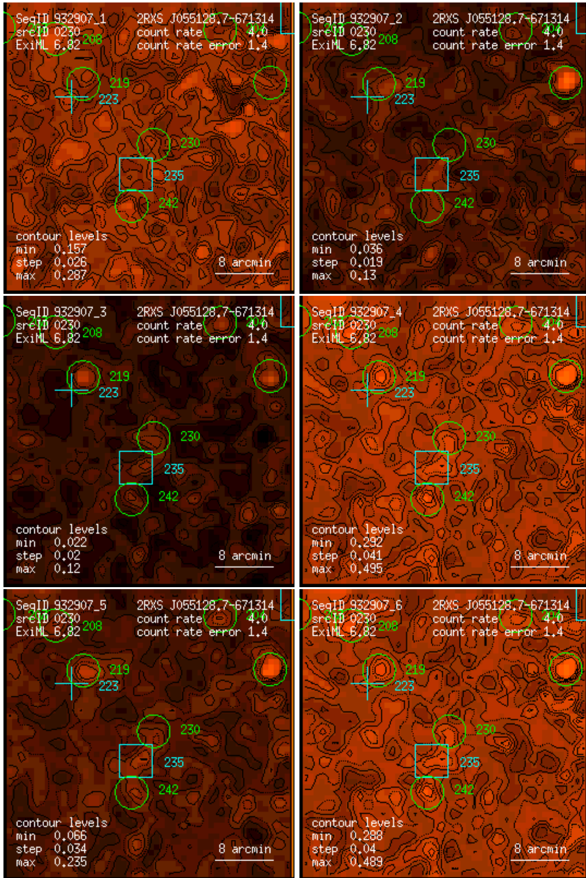
Figure 230: RASS 932907: detection 0230: band rate images, Gaussian filter: (1) PSPC channels 11 – 41, (2) 52 – 90, (3) 91 – 201, (4) 11 – 235, (5) 52 – 201, (6) 11 – 201. Broad band rates in counts/ks. Band rate contour levels in counts/ks/arcmin 2 .
