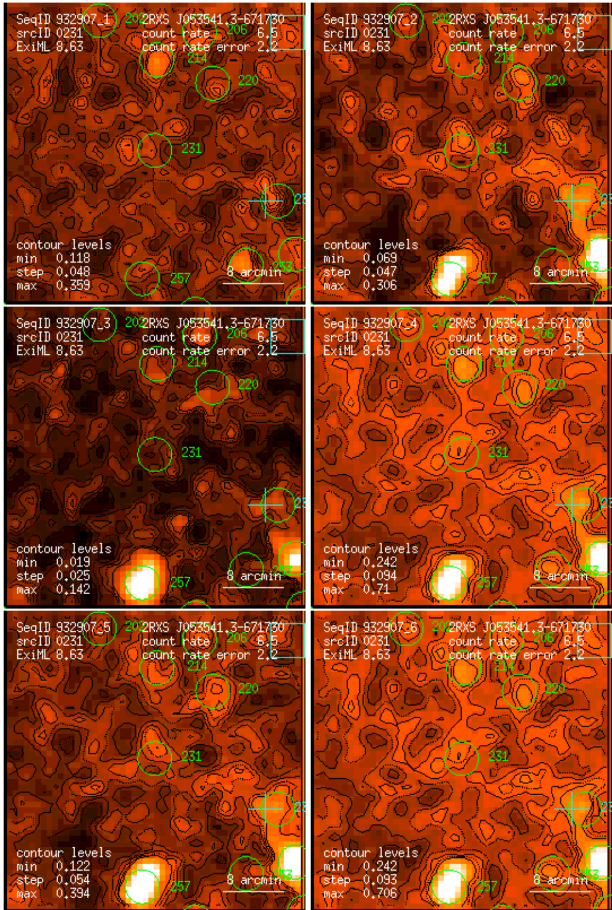
Figure 231: RASS 932907: detection 0231: band rate images, Gaussian filter: (1) PSPC channels 11 – 41, (2) 52 – 90, (3) 91 – 201, (4) 11 – 235, (5) 52 – 201, (6) 11 – 201. Broad band rates in counts/ks. Band rate contour levels in counts/ks/arcmin 2 .
