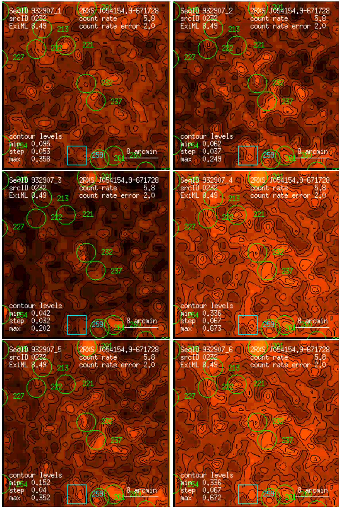
Figure 232: RASS 932907: detection 0232: band rate images, Gaussian filter: (1) PSPC channels 11 – 41, (2) 52 – 90, (3) 91 – 201, (4) 11 – 235, (5) 52 – 201, (6) 11 – 201. Broad band rates in counts/ks. Band rate contour levels in counts/ks/arcmin 2 .
