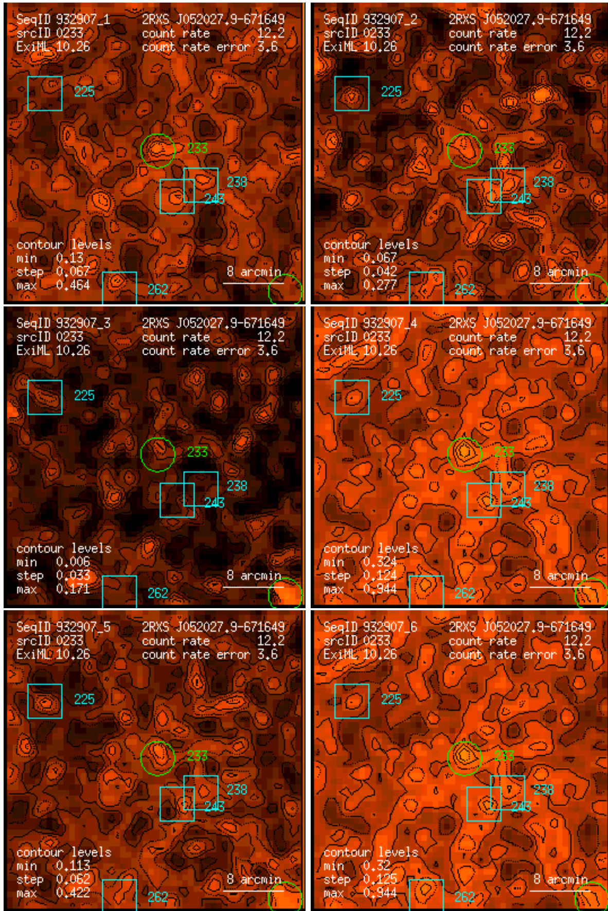
Figure 233: RASS 932907: detection 0233: band rate images, Gaussian filter: (1) PSPC channels 11 – 41, (2) 52 – 90, (3) 91 – 201, (4) 11 – 235, (5) 52 – 201, (6) 11 – 201. Broad band rates in counts/ks. Band rate contour levels in counts/ks/arcmin 2 .
