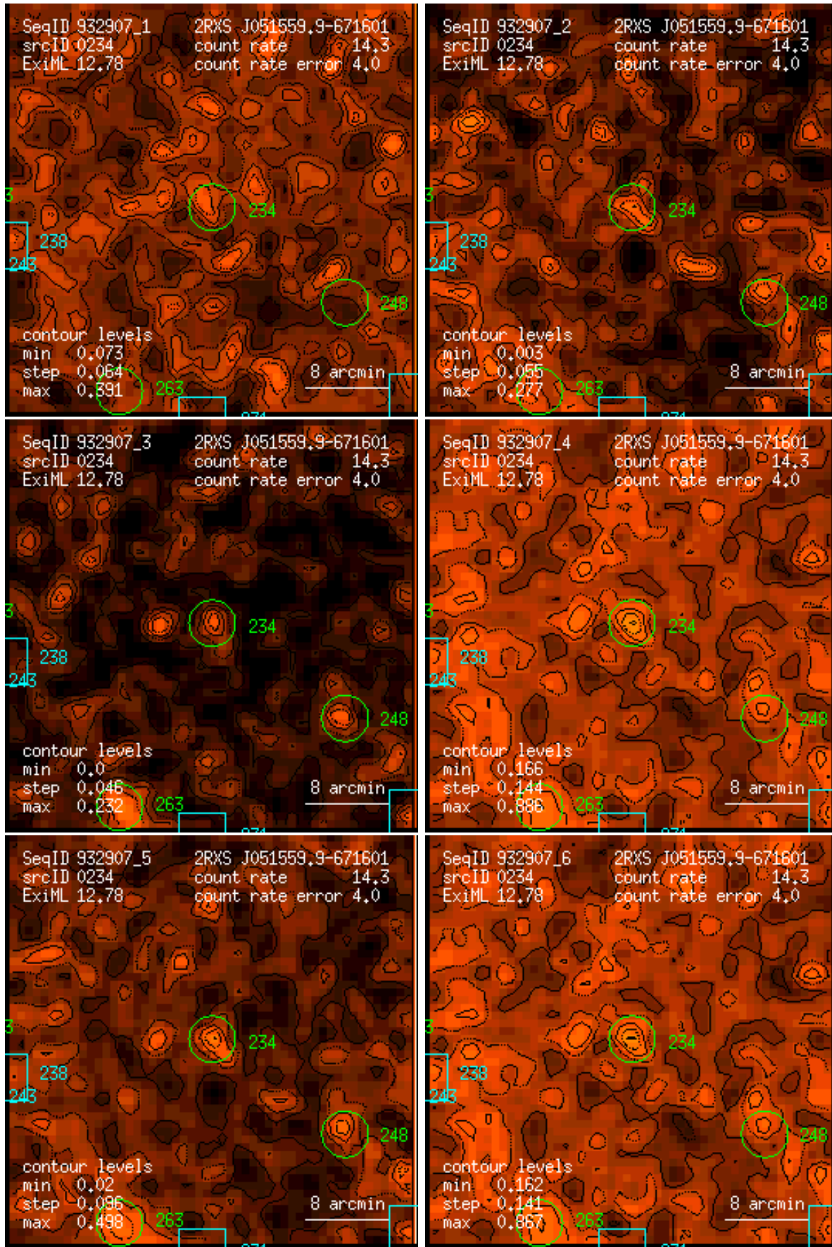
Figure 234: RASS 932907: detection 0234: band rate images, Gaussian filter: (1) PSPC channels 11 – 41, (2) 52 – 90, (3) 91 – 201, (4) 11 – 235, (5) 52 – 201, (6) 11 – 201. Broad band rates in counts/ks. Band rate contour levels in counts/ks/arcmin 2 .
