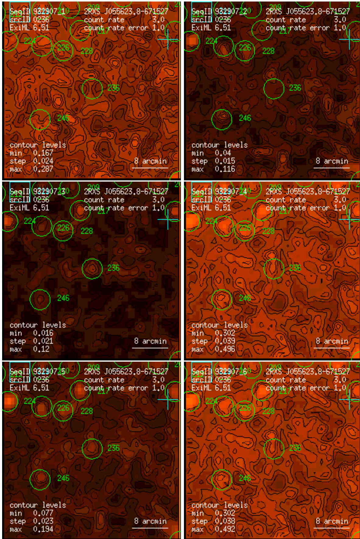
Figure 236: RASS 932907: detection 0236: band rate images, Gaussian filter: (1) PSPC channels 11 – 41, (2) 52 – 90, (3) 91 – 201, (4) 11 – 235, (5) 52 – 201, (6) 11 – 201. Broad band rates in counts/ks. Band rate contour levels in counts/ks/arcmin 2 .
