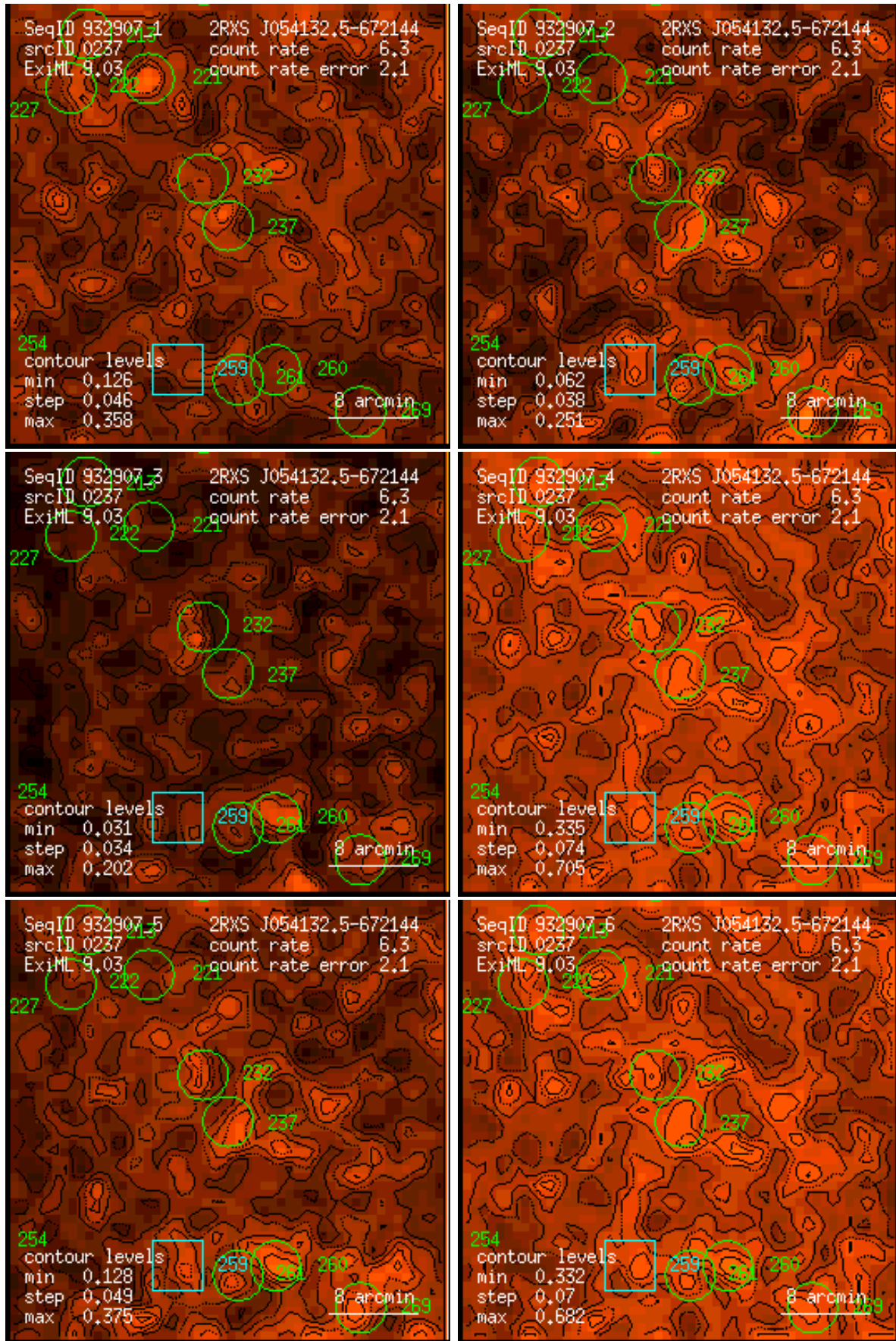
Figure 237: RASS 932907: detection 0237: band rate images, Gaussian filter: (1) PSPC channels 11 – 41, (2) 52 – 90, (3) 91 – 201, (4) 11 – 235, (5) 52 – 201, (6) 11 – 201. Broad band rates in counts/ks. Band rate contour levels in counts/ks/arcmin 2 .
