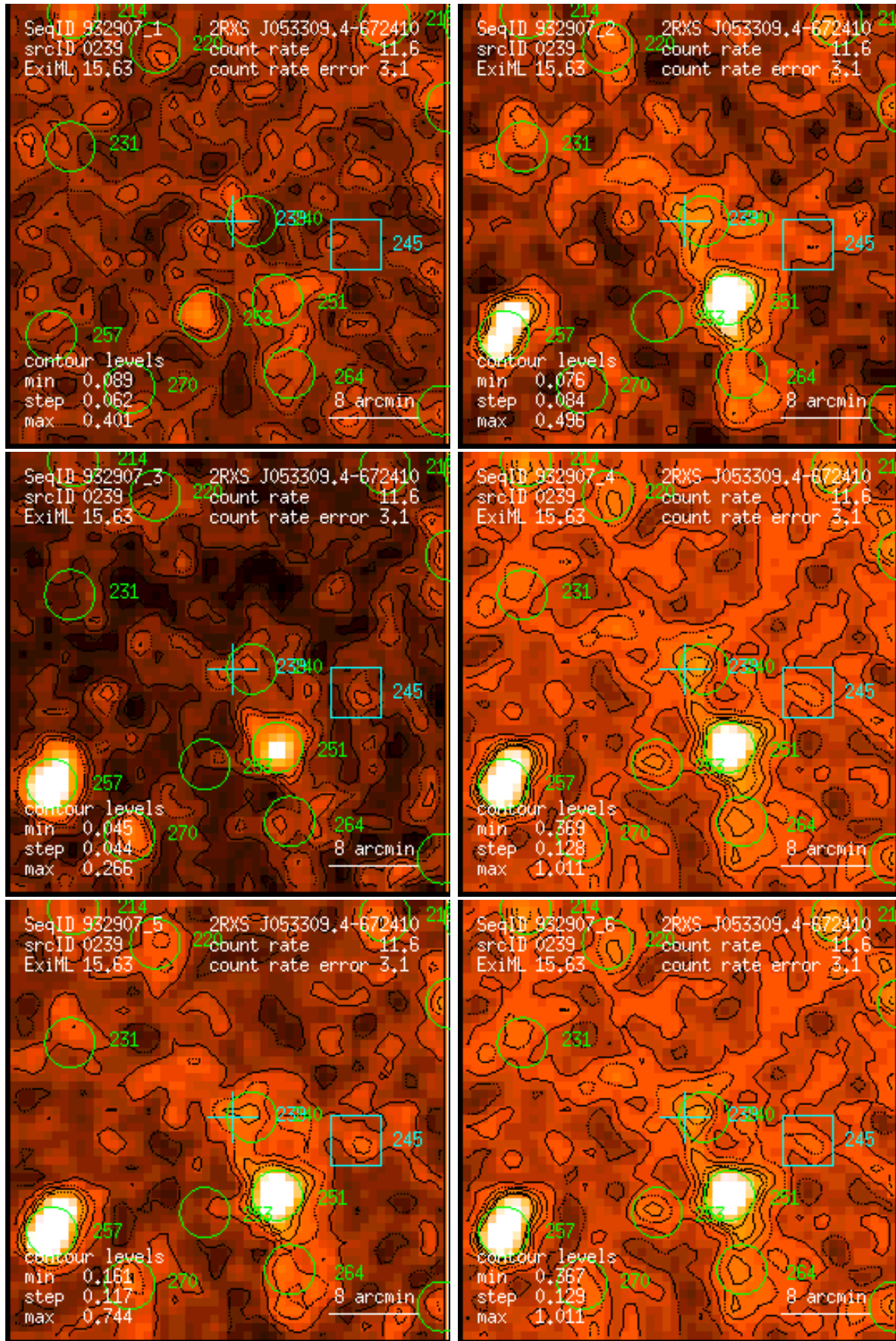
Figure 239: RASS 932907: detection 0239: band rate images, Gaussian filter: (1) PSPC channels 11 – 41, (2) 52 – 90, (3) 91 – 201, (4) 11 – 235, (5) 52 – 201, (6) 11 – 201. Broad band rates in counts/ks. Band rate contour levels in counts/ks/arcmin 2 .
