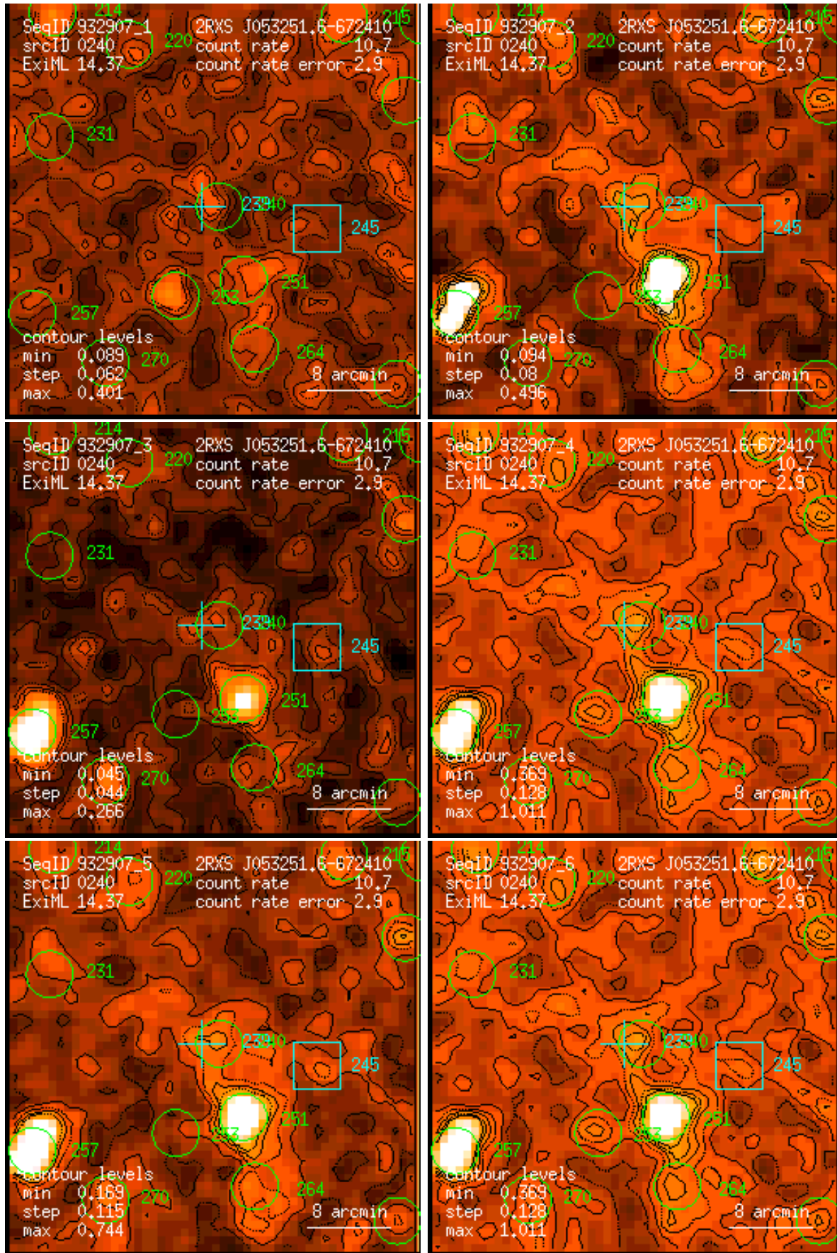
Figure 240: RASS 932907: detection 0240: band rate images, Gaussian filter: (1) PSPC channels 11 – 41, (2) 52 – 90, (3) 91 – 201, (4) 11 – 235, (5) 52 – 201, (6) 11 – 201. Broad band rates in counts/ks. Band rate contour levels in counts/ks/arcmin 2 .
