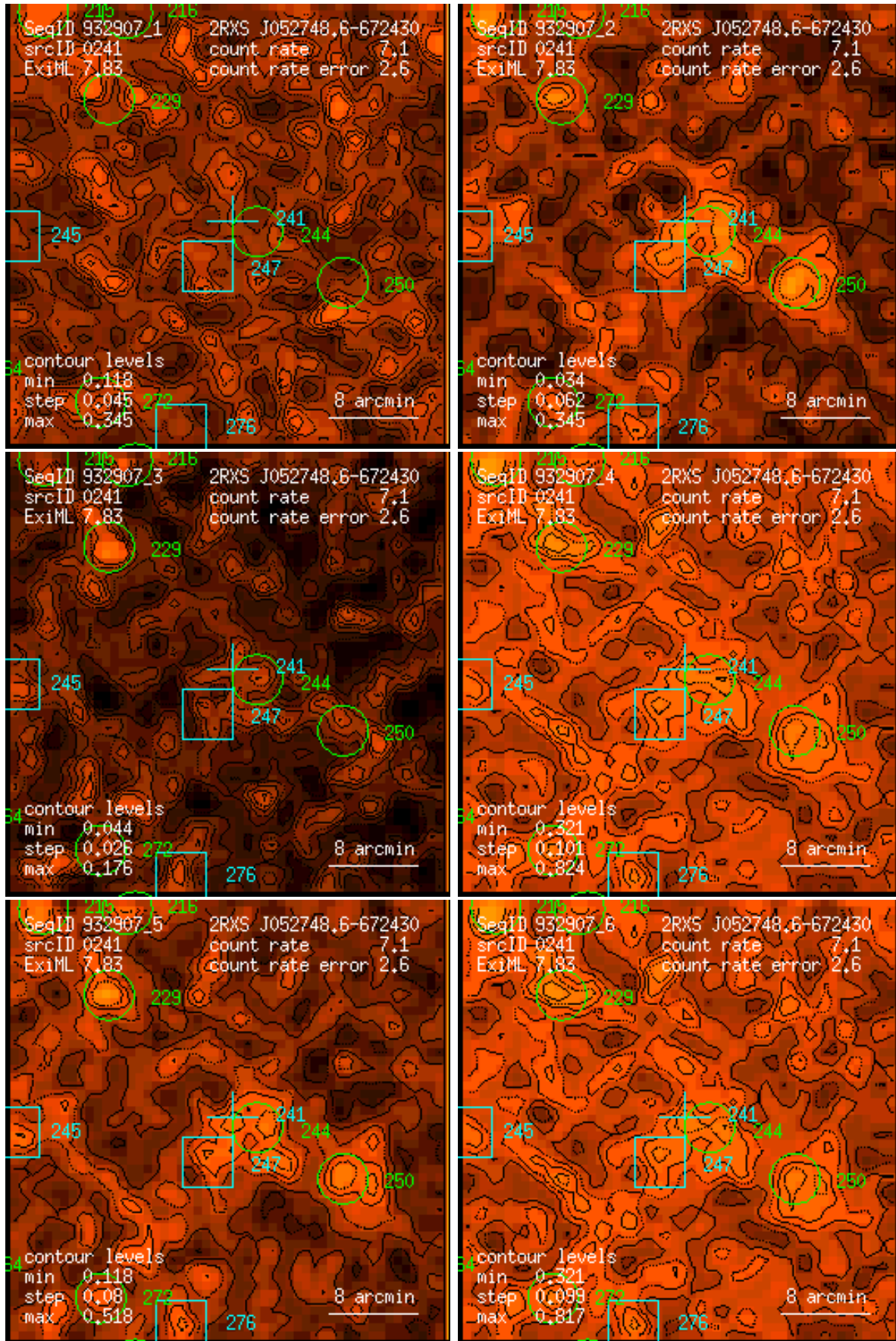
Figure 241: RASS 932907: detection 0241: band rate images, Gaussian filter: (1) PSPC channels 11 – 41, (2) 52 – 90, (3) 91 – 201, (4) 11 – 235, (5) 52 – 201, (6) 11 – 201. Broad band rates in counts/ks. Band rate contour levels in counts/ks/arcmin 2 .
