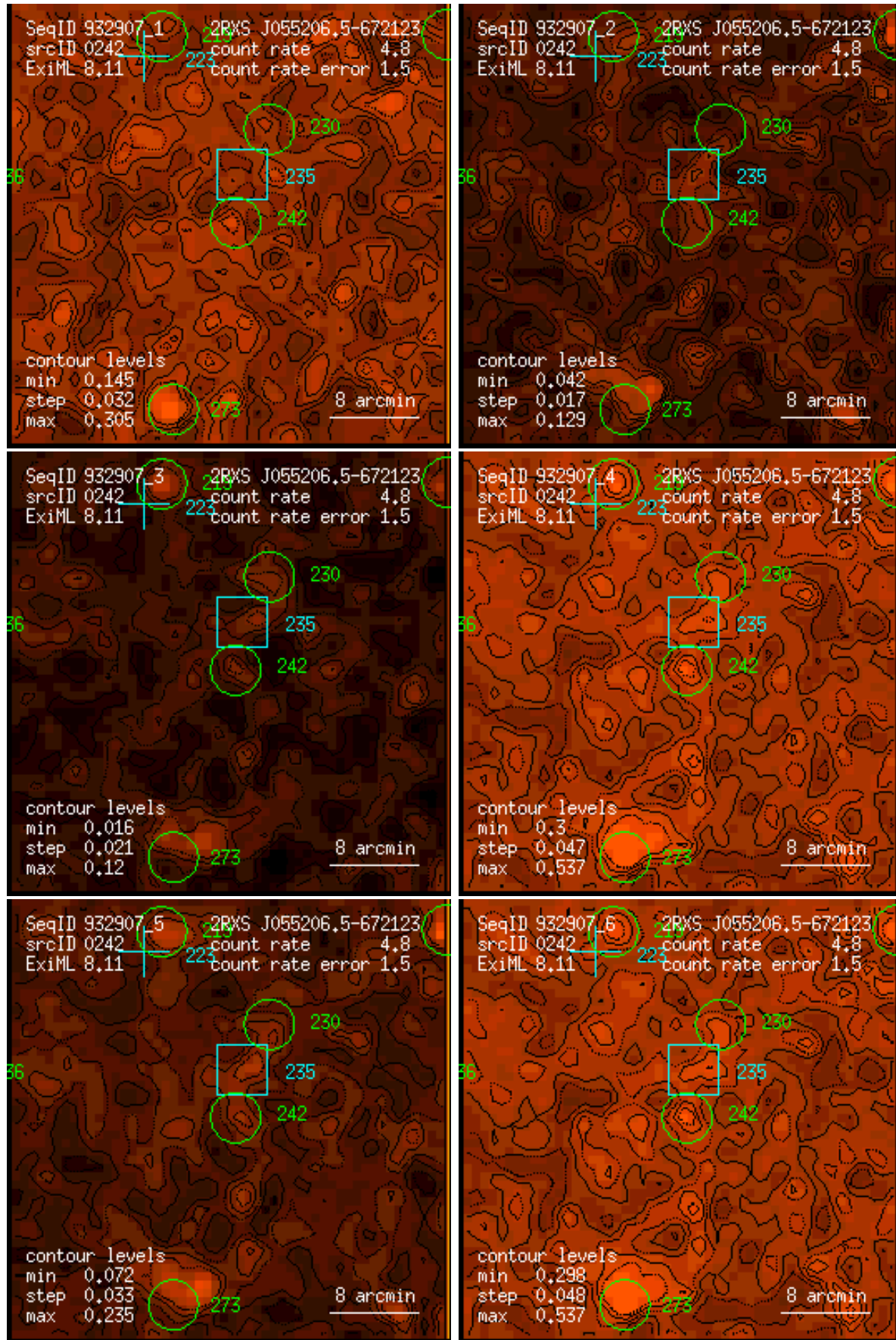
Figure 242: RASS 932907: detection 0242: band rate images, Gaussian filter: (1) PSPC channels 11 – 41, (2) 52 – 90, (3) 91 – 201, (4) 11 – 235, (5) 52 – 201, (6) 11 – 201. Broad band rates in counts/ks. Band rate contour levels in counts/ks/arcmin 2 .
