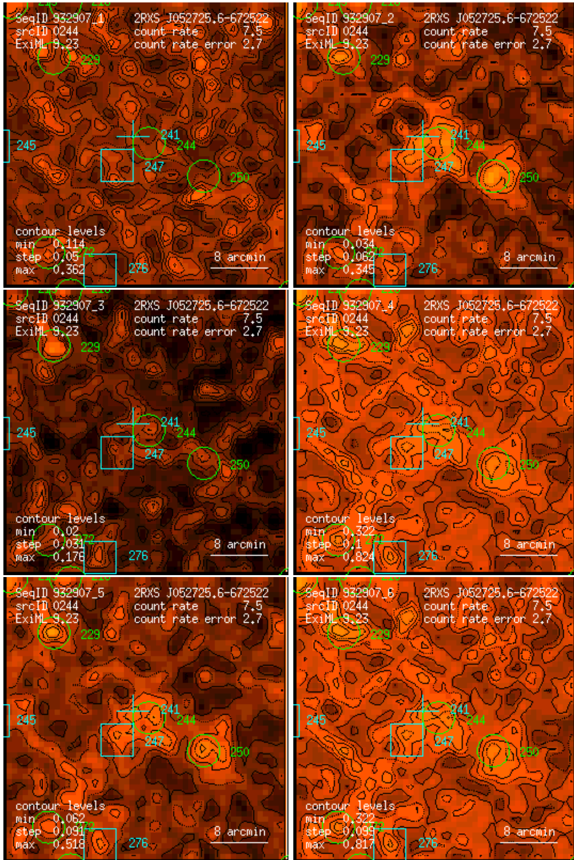
Figure 244: RASS 932907: detection 0244: band rate images, Gaussian filter: (1) PSPC channels 11 – 41, (2) 52 – 90, (3) 91 – 201, (4) 11 – 235, (5) 52 – 201, (6) 11 – 201. Broad band rates in counts/ks. Band rate contour levels in counts/ks/arcmin 2 .
