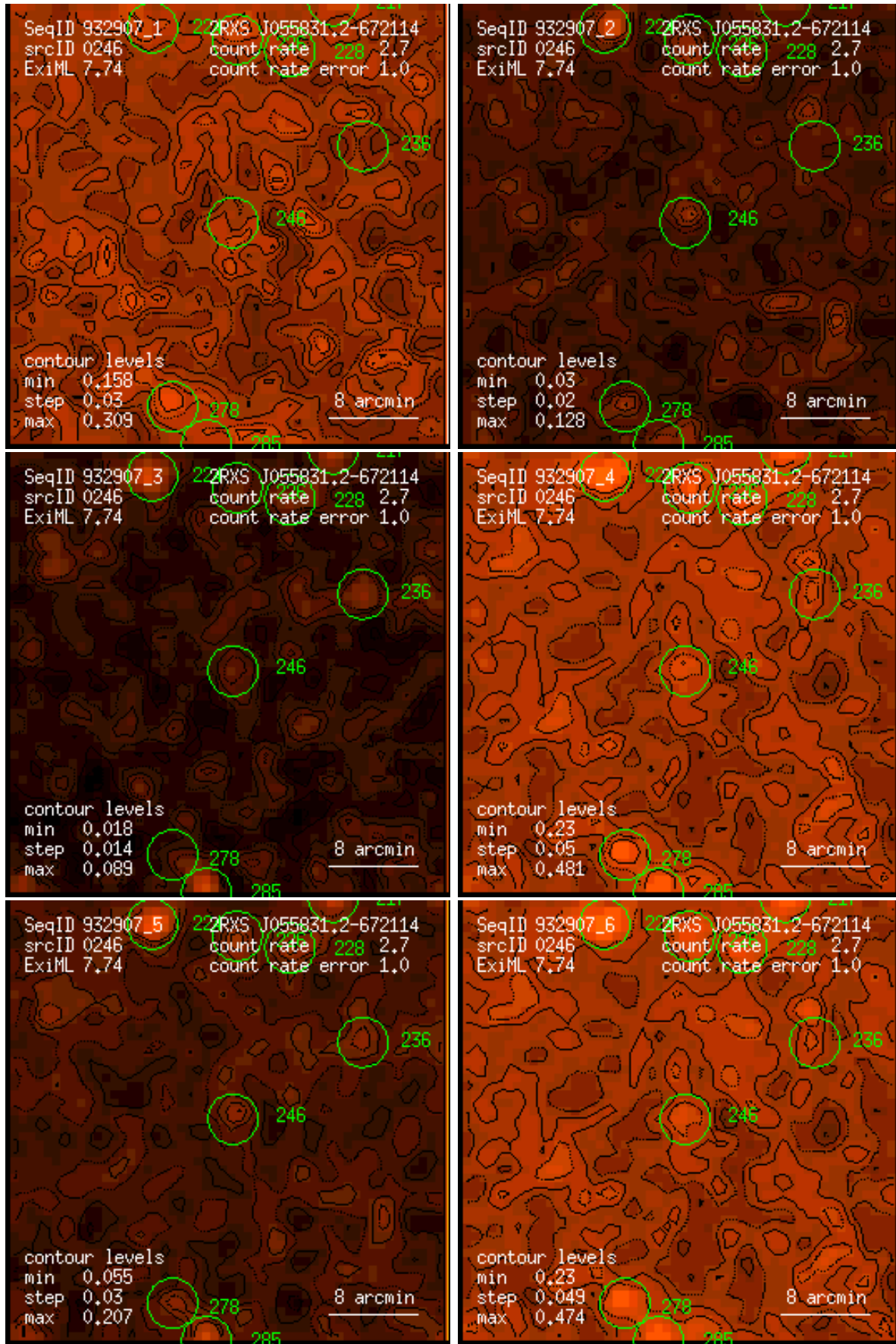
Figure 246: RASS 932907: detection 0246: band rate images, Gaussian filter: (1) PSPC channels 11 – 41, (2) 52 – 90, (3) 91 – 201, (4) 11 – 235, (5) 52 – 201, (6) 11 – 201. Broad band rates in counts/ks. Band rate contour levels in counts/ks/arcmin 2 .
