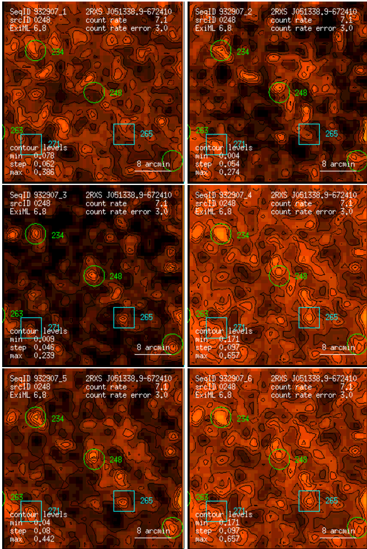
Figure 248: RASS 932907: detection 0248: band rate images, Gaussian filter: (1) PSPC channels 11 – 41, (2) 52 – 90, (3) 91 – 201, (4) 11 – 235, (5) 52 – 201, (6) 11 – 201. Broad band rates in counts/ks. Band rate contour levels in counts/ks/arcmin 2 .
