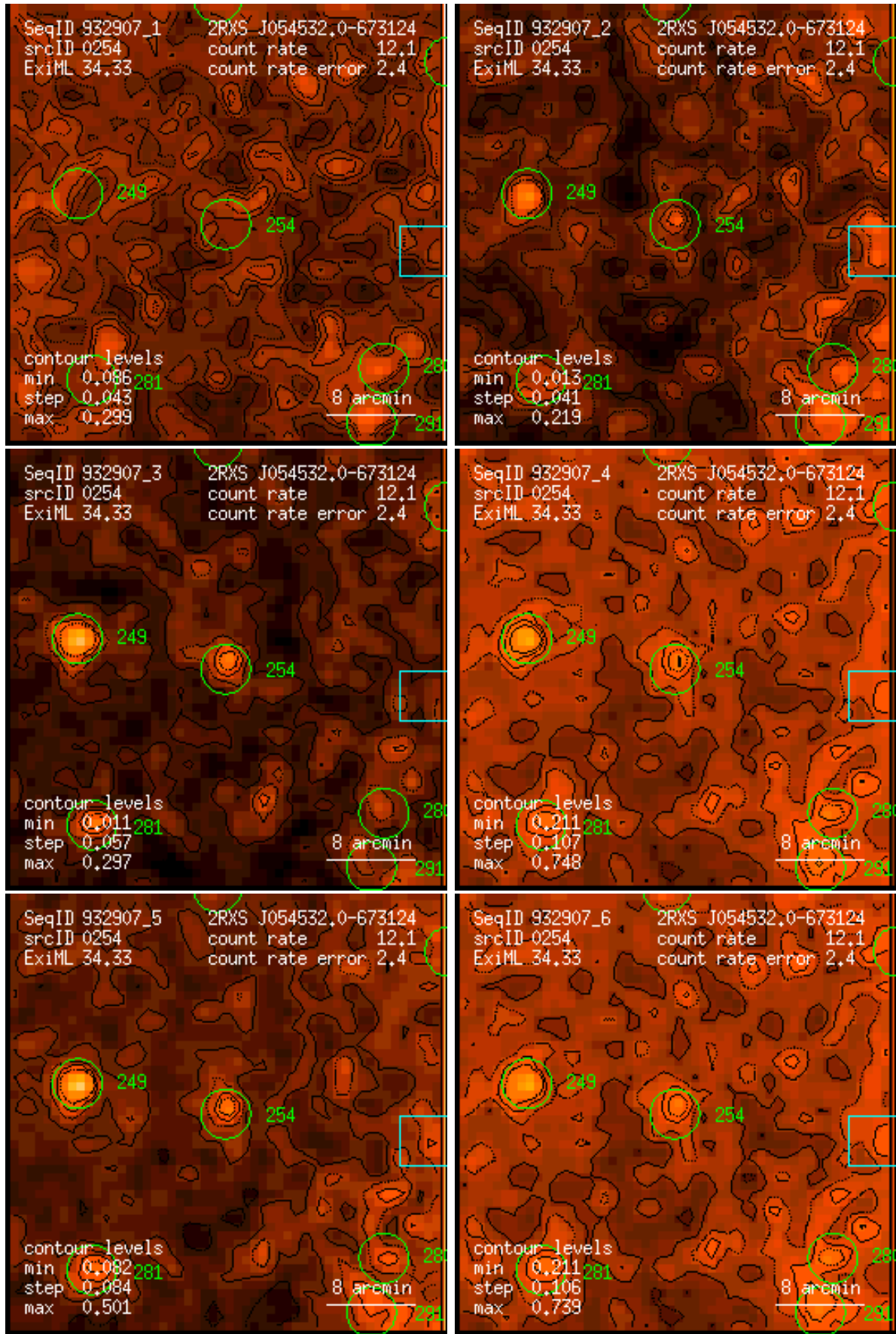
Figure 254: RASS 932907: detection 0254: band rate images, Gaussian filter: (1) PSPC channels 11 – 41, (2) 52 – 90, (3) 91 – 201, (4) 11 – 235, (5) 52 – 201, (6) 11 – 201. Broad band rates in counts/ks. Band rate contour levels in counts/ks/arcmin 2 .
