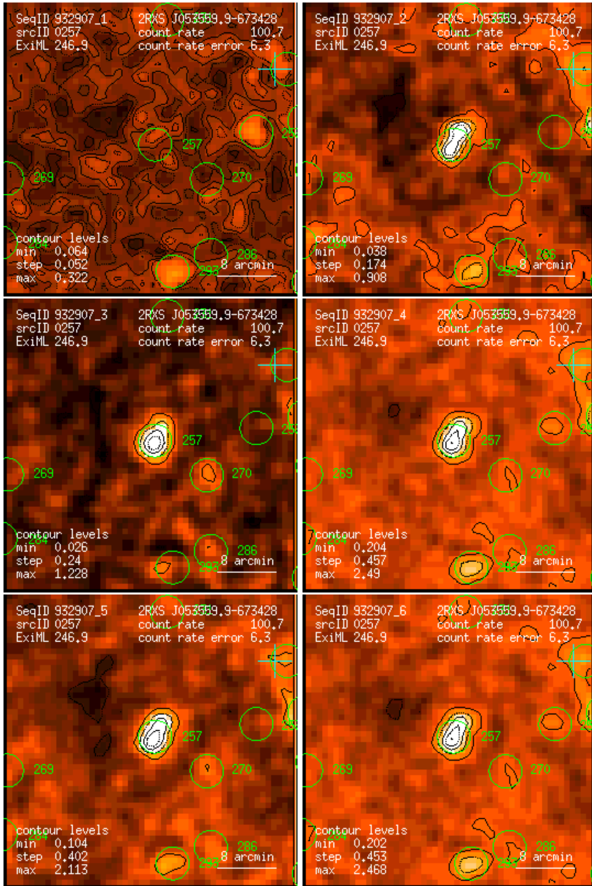
Figure 257: RASS 932907: detection 0257: band rate images, Gaussian filter: (1) PSPC channels 11 – 41, (2) 52 – 90, (3) 91 – 201, (4) 11 – 235, (5) 52 – 201, (6) 11 – 201. Broad band rates in counts/ks. Band rate contour levels in counts/ks/arcmin 2 .
