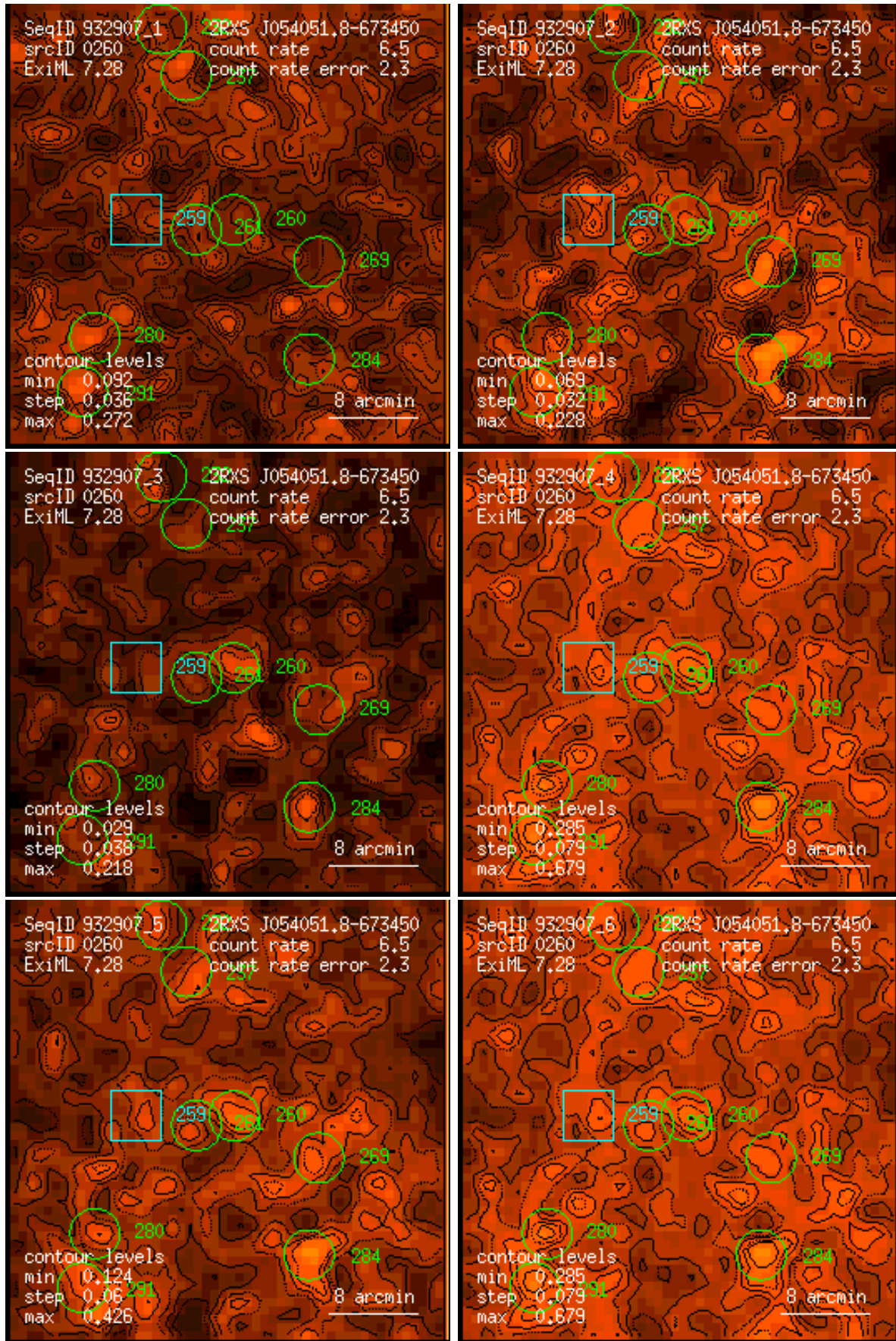
Figure 260: RASS 932907: detection 0260: band rate images, Gaussian filter: (1) PSPC channels 11 – 41, (2) 52 – 90, (3) 91 – 201, (4) 11 – 235, (5) 52 – 201, (6) 11 – 201. Broad band rates in counts/ks. Band rate contour levels in counts/ks/arcmin 2 .
