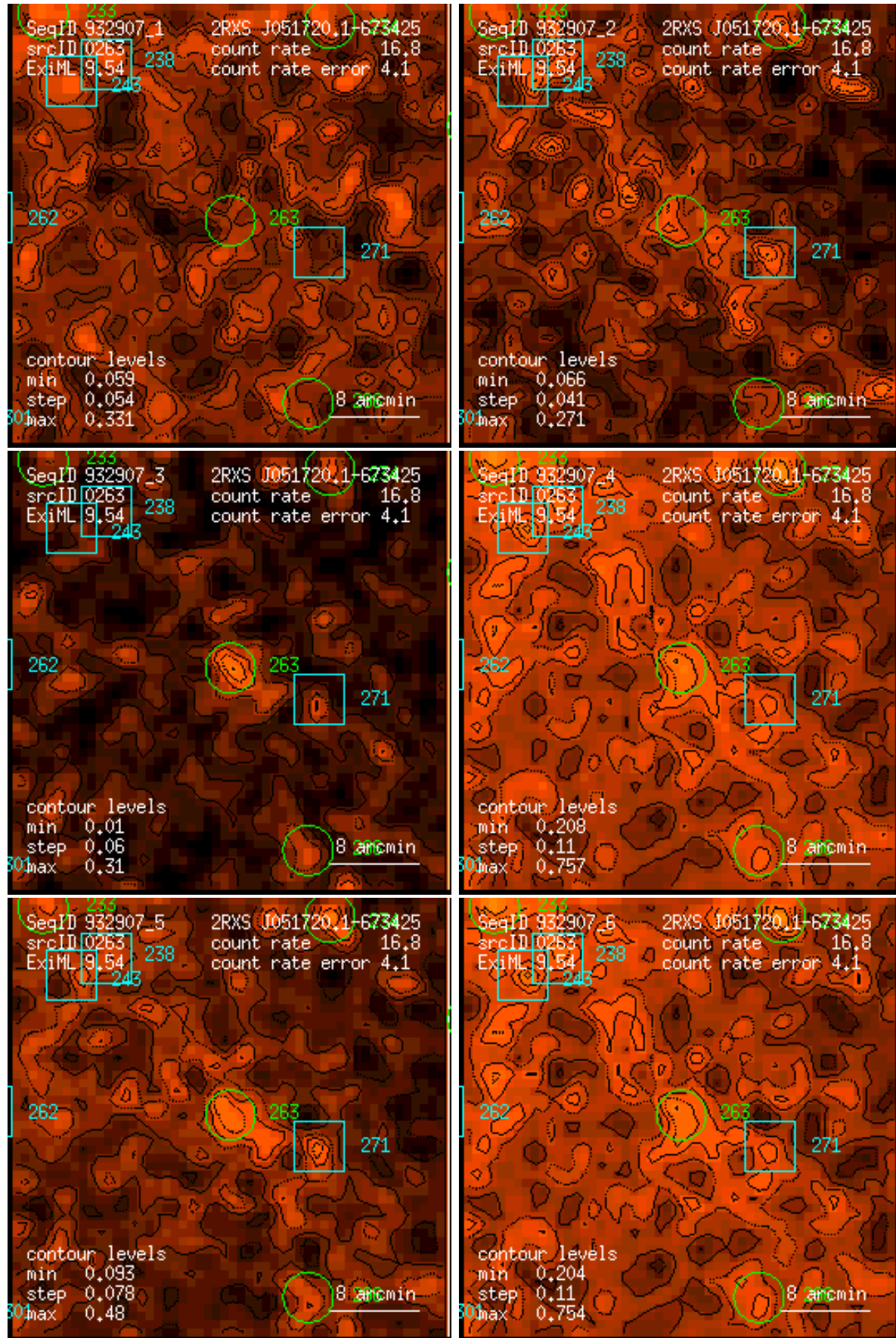
Figure 263: RASS 932907: detection 0263: band rate images, Gaussian filter: (1) PSPC channels 11 – 41, (2) 52 – 90, (3) 91 – 201, (4) 11 – 235, (5) 52 – 201, (6) 11 – 201. Broad band rates in counts/ks. Band rate contour levels in counts/ks/arcmin 2 .
