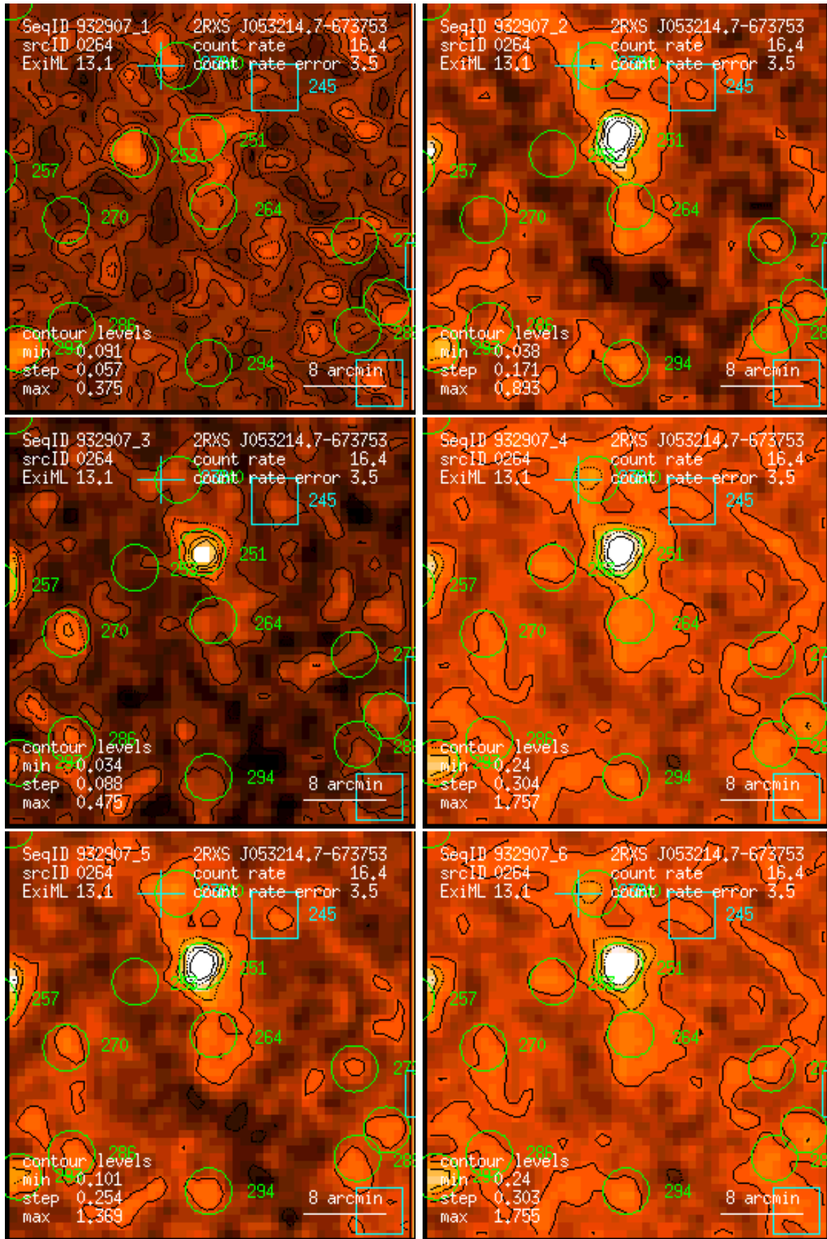
Figure 264: RASS 932907: detection 0264: band rate images, Gaussian filter: (1) PSPC channels 11 – 41, (2) 52 – 90, (3) 91 – 201, (4) 11 – 235, (5) 52 – 201, (6) 11 – 201. Broad band rates in counts/ks. Band rate contour levels in counts/ks/arcmin 2 .
