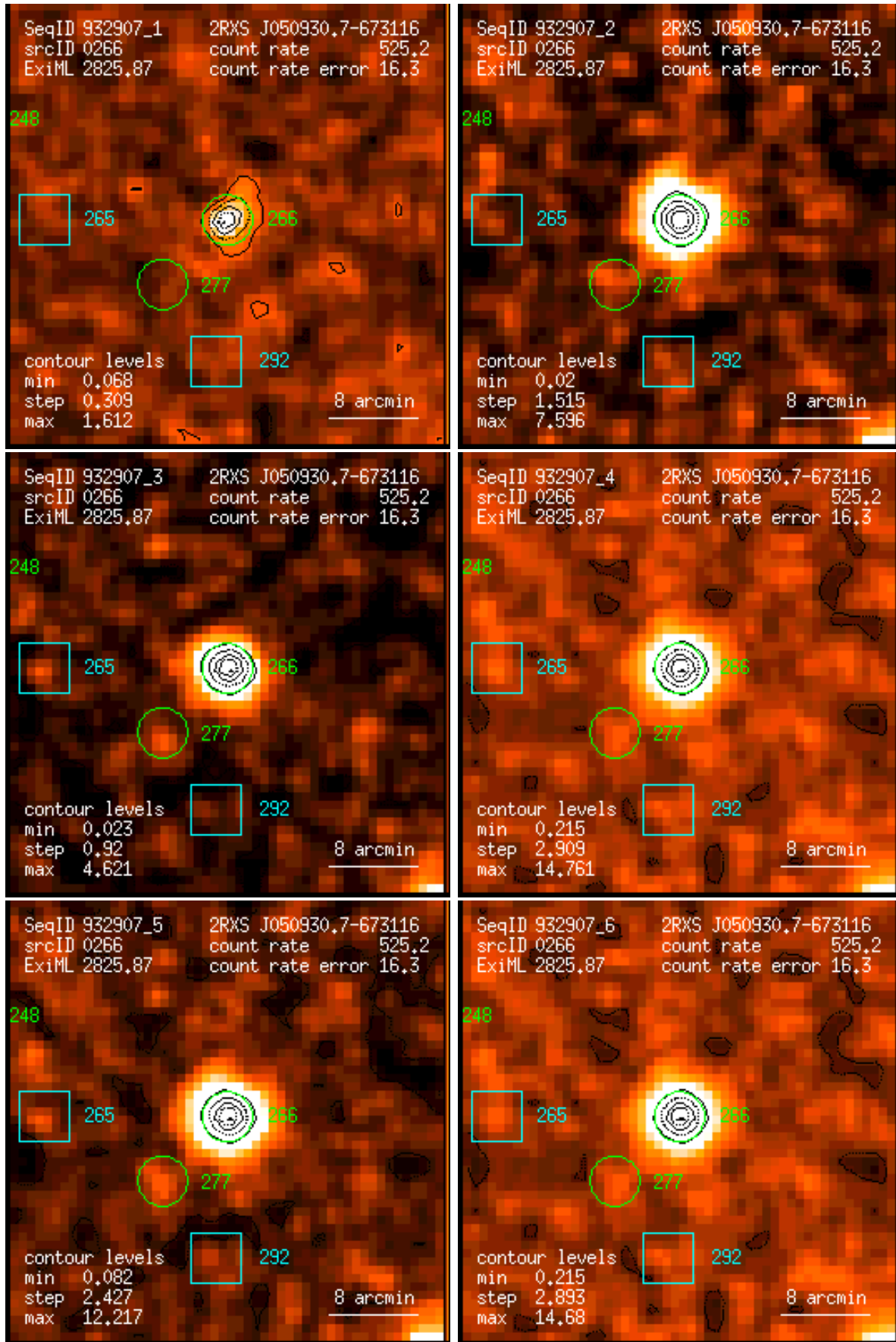
Figure 266: RASS 932907: detection 0266: band rate images, Gaussian filter: (1) PSPC channels 11 – 41, (2) 52 – 90, (3) 91 – 201, (4) 11 – 235, (5) 52 – 201, (6) 11 – 201. Broad band rates in counts/ks. Band rate contour levels in counts/ks/arcmin 2 .
