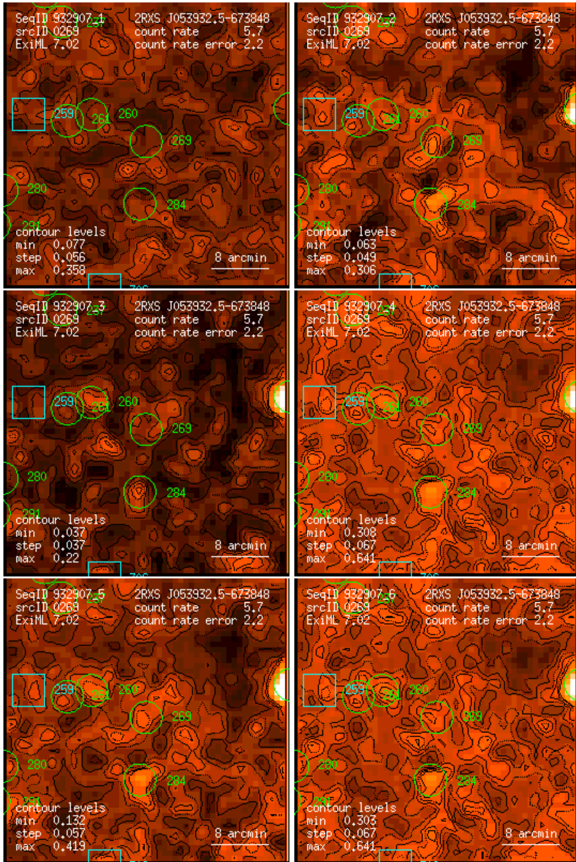
Figure 269: RASS 932907: detection 0269: band rate images, Gaussian filter: (1) PSPC channels 11 – 41, (2) 52 – 90, (3) 91 – 201, (4) 11 – 235, (5) 52 – 201, (6) 11 – 201. Broad band rates in counts/ks. Band rate contour levels in counts/ks/arcmin 2 .
