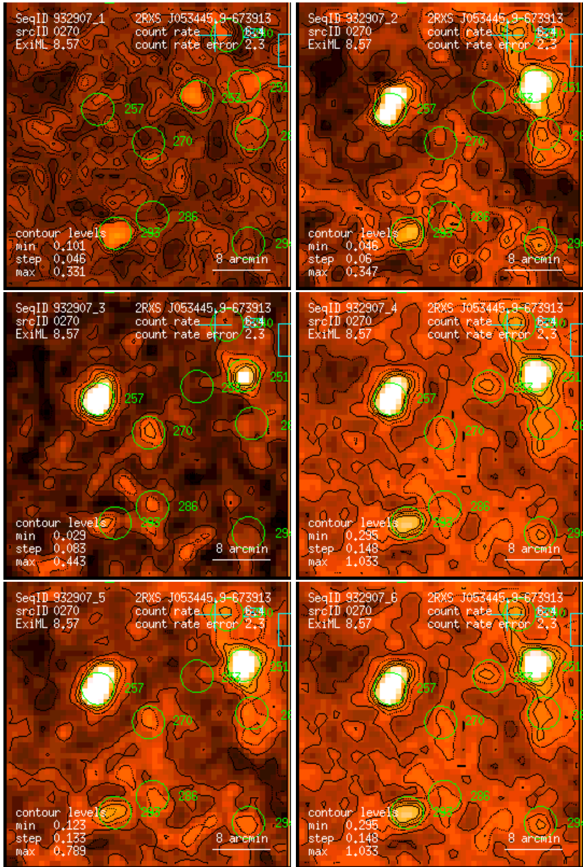
Figure 270: RASS 932907: detection 0270: band rate images, Gaussian filter: (1) PSPC channels 11 – 41, (2) 52 – 90, (3) 91 – 201, (4) 11 – 235, (5) 52 – 201, (6) 11 – 201. Broad band rates in counts/ks. Band rate contour levels in counts/ks/arcmin 2 .
