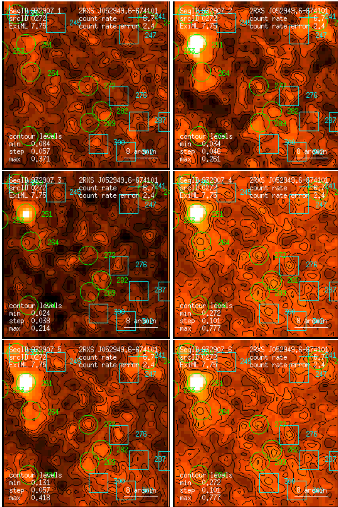
Figure 272: RASS 932907: detection 0272: band rate images, Gaussian filter: (1) PSPC channels 11 – 41, (2) 52 – 90, (3) 91 – 201, (4) 11 – 235, (5) 52 – 201, (6) 11 – 201. Broad band rates in counts/ks. Band rate contour levels in counts/ks/arcmin 2 .
