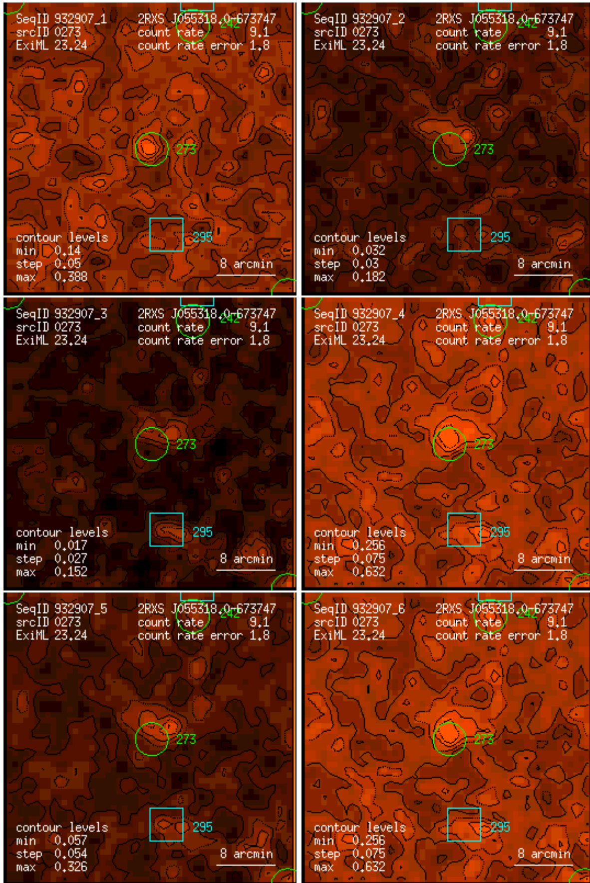
Figure 273: RASS 932907: detection 0273: band rate images, Gaussian filter: (1) PSPC channels 11 – 41, (2) 52 – 90, (3) 91 – 201, (4) 11 – 235, (5) 52 – 201, (6) 11 – 201. Broad band rates in counts/ks. Band rate contour levels in counts/ks/arcmin 2 .
