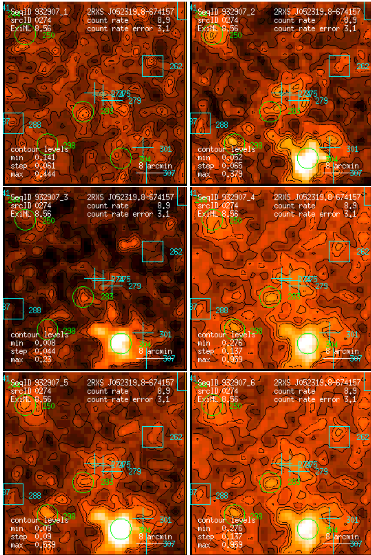
Figure 274: RASS 932907: detection 0274: band rate images, Gaussian filter: (1) PSPC channels 11 – 41, (2) 52 – 90, (3) 91 – 201, (4) 11 – 235, (5) 52 – 201, (6) 11 – 201. Broad band rates in counts/ks. Band rate contour levels in counts/ks/arcmin 2 .
